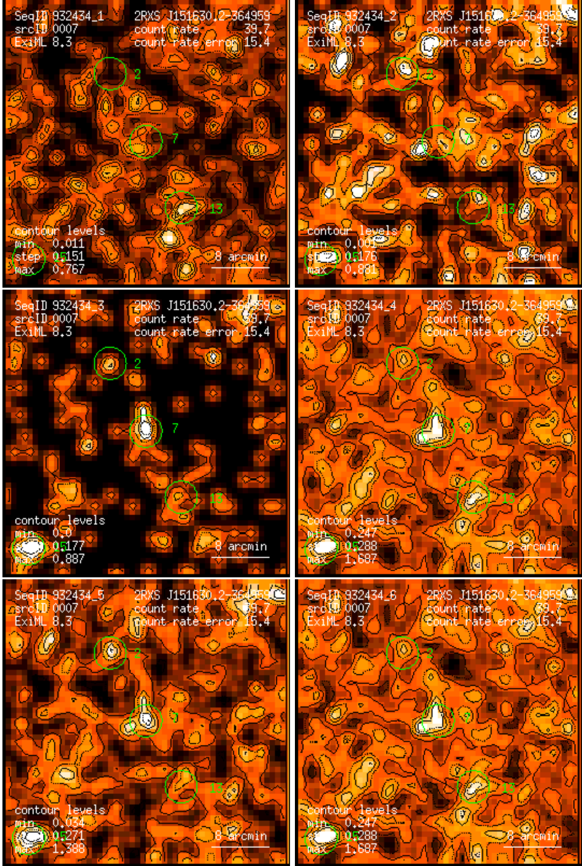
Figure 7: RASS 932434: detection 0007: band rate images, Gaussian filter: (1) PSPC channels 11 – 41, (2) 52 – 90, (3) 91 – 201, (4) 11 – 235, (5) 52 – 201, (6) 11 – 201. Broad band rates in counts/ks. Band rate contour levels in counts/ks/arcmin 2 .
