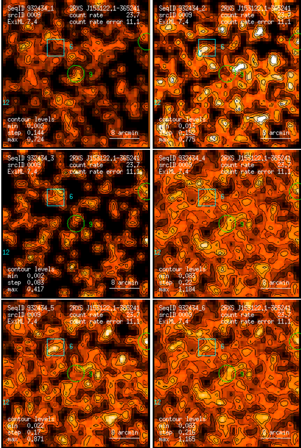
Figure 9: RASS 932434: detection 0009: band rate images, Gaussian filter: (1) PSPC channels 11 – 41, (2) 52 – 90, (3) 91 – 201, (4) 11 – 235, (5) 52 – 201, (6) 11 – 201. Broad band rates in counts/ks. Band rate contour levels in counts/ks/arcmin 2 .
