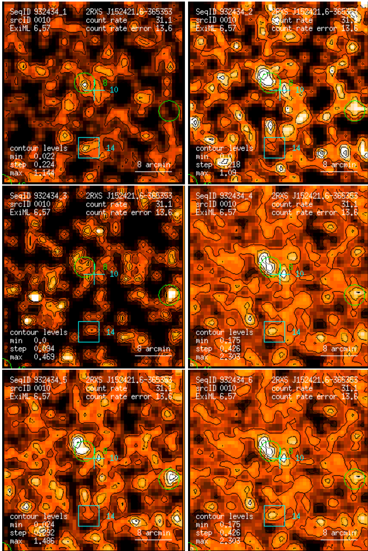
Figure 10: RASS 932434: detection 0010: band rate images, Gaussian filter: (1) PSPC channels 11 – 41, (2) 52 – 90, (3) 91 – 201, (4) 11 – 235, (5) 52 – 201, (6) 11 – 201. Broad band rates in counts/ks. Band rate contour levels in counts/ks/arcmin 2 .
