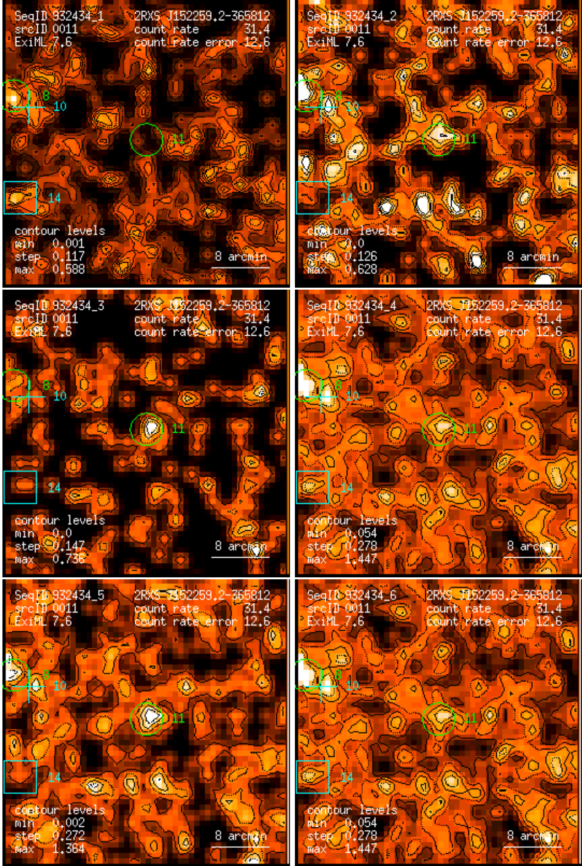
Figure 11: RASS 932434: detection 0011: band rate images, Gaussian filter: (1) PSPC channels 11 – 41, (2) 52 – 90, (3) 91 – 201, (4) 11 – 235, (5) 52 – 201, (6) 11 – 201. Broad band rates in counts/ks. Band rate contour levels in counts/ks/arcmin 2 .
