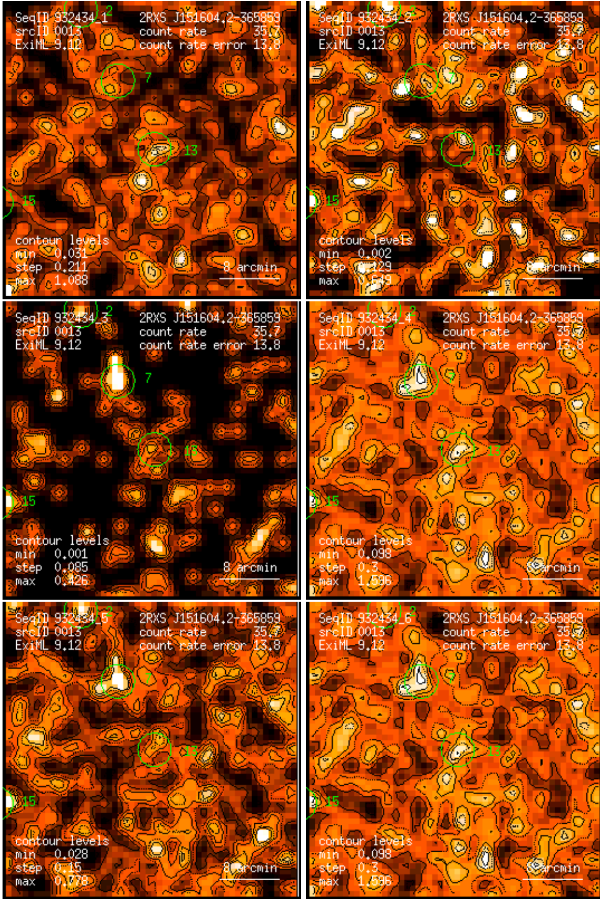
Figure 13: RASS 932434: detection 0013: band rate images, Gaussian filter: (1) PSPC channels 11 – 41, (2) 52 – 90, (3) 91 – 201, (4) 11 – 235, (5) 52 – 201, (6) 11 – 201. Broad band rates in counts/ks. Band rate contour levels in counts/ks/arcmin 2 .
