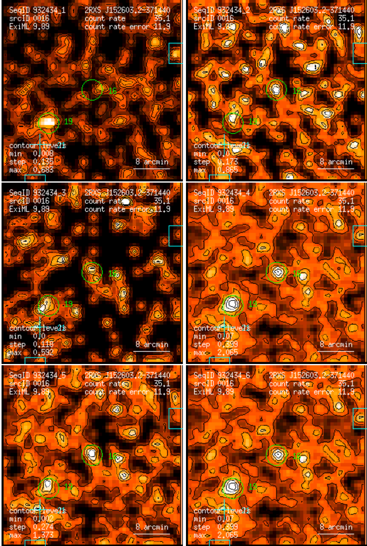
Figure 16: RASS 932434: detection 0016: band rate images, Gaussian filter: (1) PSPC channels 11 – 41, (2) 52 – 90, (3) 91 – 201, (4) 11 – 235, (5) 52 – 201, (6) 11 – 201. Broad band rates in counts/ks. Band rate contour levels in counts/ks/arcmin 2 .
