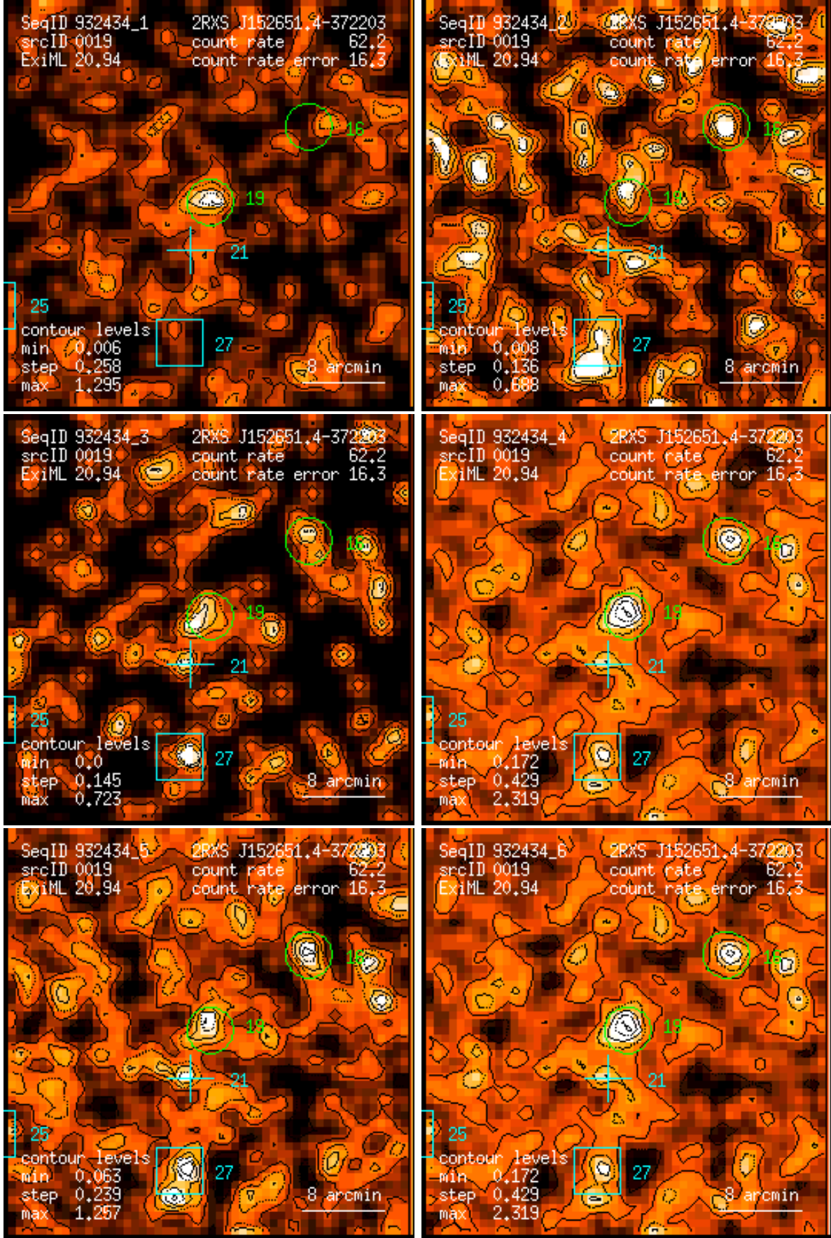
Figure 19: RASS 932434: detection 0019: band rate images, Gaussian filter: (1) PSPC channels 11 – 41, (2) 52 – 90, (3) 91 – 201, (4) 11 – 235, (5) 52 – 201, (6) 11 – 201. Broad band rates in counts/ks. Band rate contour levels in counts/ks/arcmin 2 .
