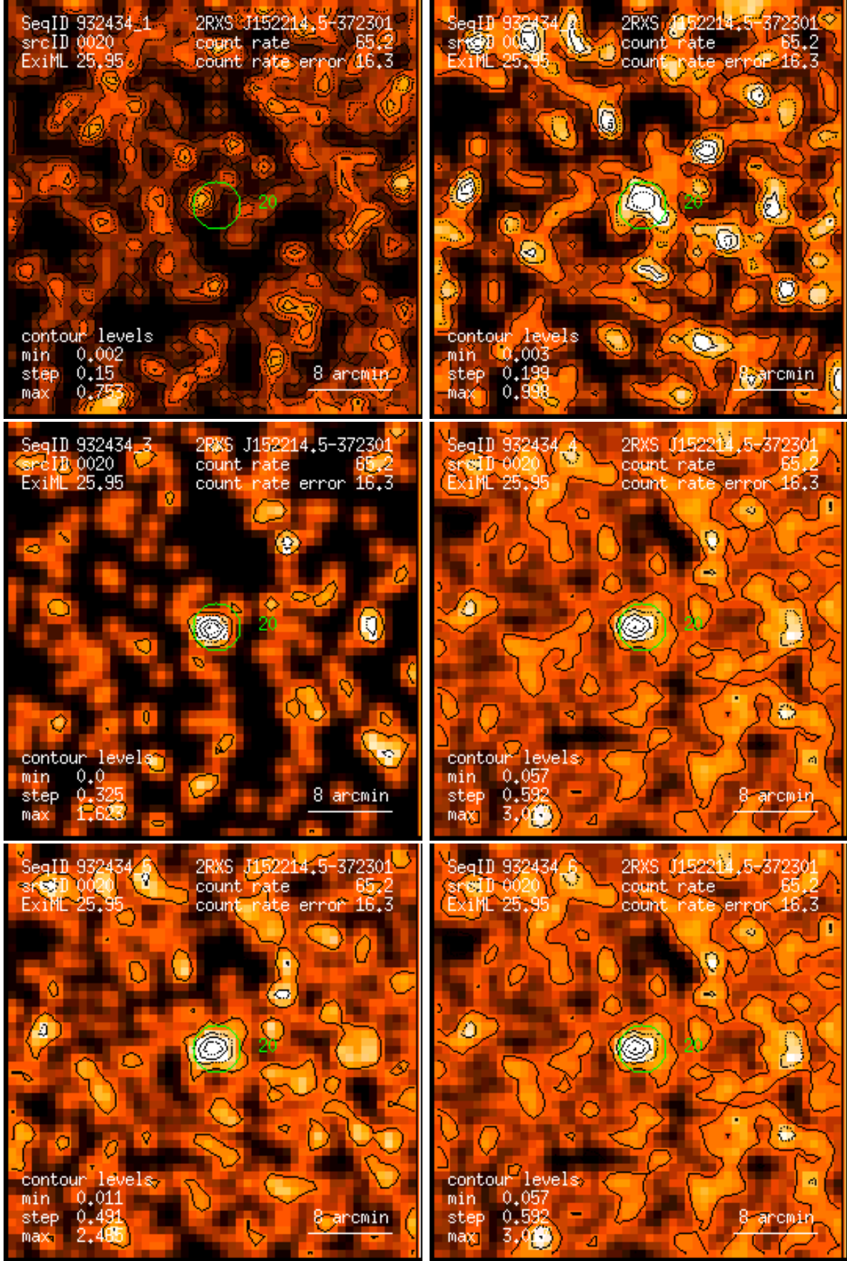
Figure 20: RASS 932434: detection 0020: band rate images, Gaussian filter: (1) PSPC channels 11 – 41, (2) 52 – 90, (3) 91 – 201, (4) 11 – 235, (5) 52 – 201, (6) 11 – 201. Broad band rates in counts/ks. Band rate contour levels in counts/ks/arcmin 2 .
