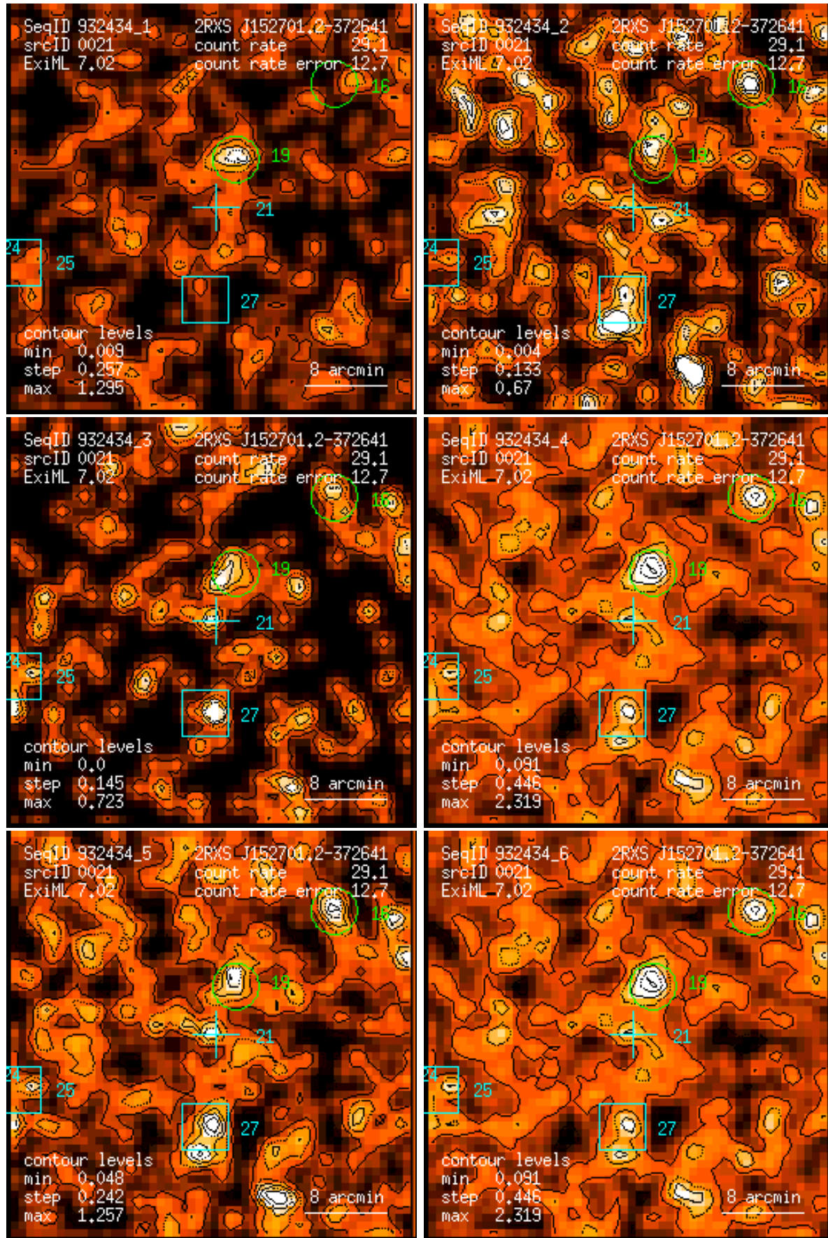
Figure 21: RASS 932434: detection 0021: band rate images, Gaussian filter: (1) PSPC channels 11 – 41, (2) 52 – 90, (3) 91 – 201, (4) 11 – 235, (5) 52 – 201, (6) 11 – 201. Broad band rates in counts/ks. Band rate contour levels in counts/ks/arcmin 2 .
