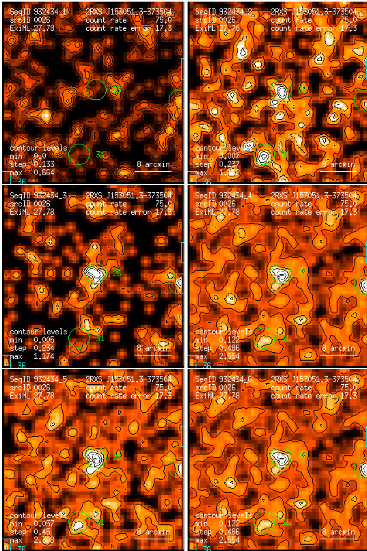
Figure 26: RASS 932434: detection 0026: band rate images, Gaussian filter: (1) PSPC channels 11 – 41, (2) 52 – 90, (3) 91 – 201, (4) 11 – 235, (5) 52 – 201, (6) 11 – 201. Broad band rates in counts/ks. Band rate contour levels in counts/ks/arcmin 2 .
