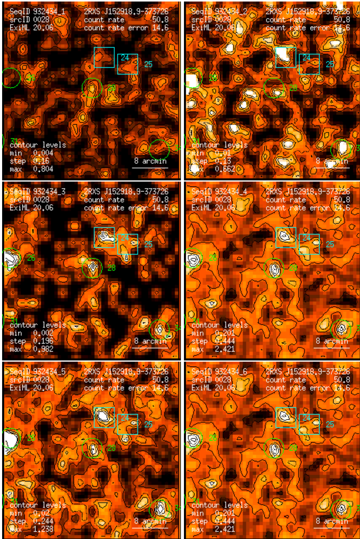
Figure 28: RASS 932434: detection 0028: band rate images, Gaussian filter: (1) PSPC channels 11 – 41, (2) 52 – 90, (3) 91 – 201, (4) 11 – 235, (5) 52 – 201, (6) 11 – 201. Broad band rates in counts/ks. Band rate contour levels in counts/ks/arcmin 2 .
