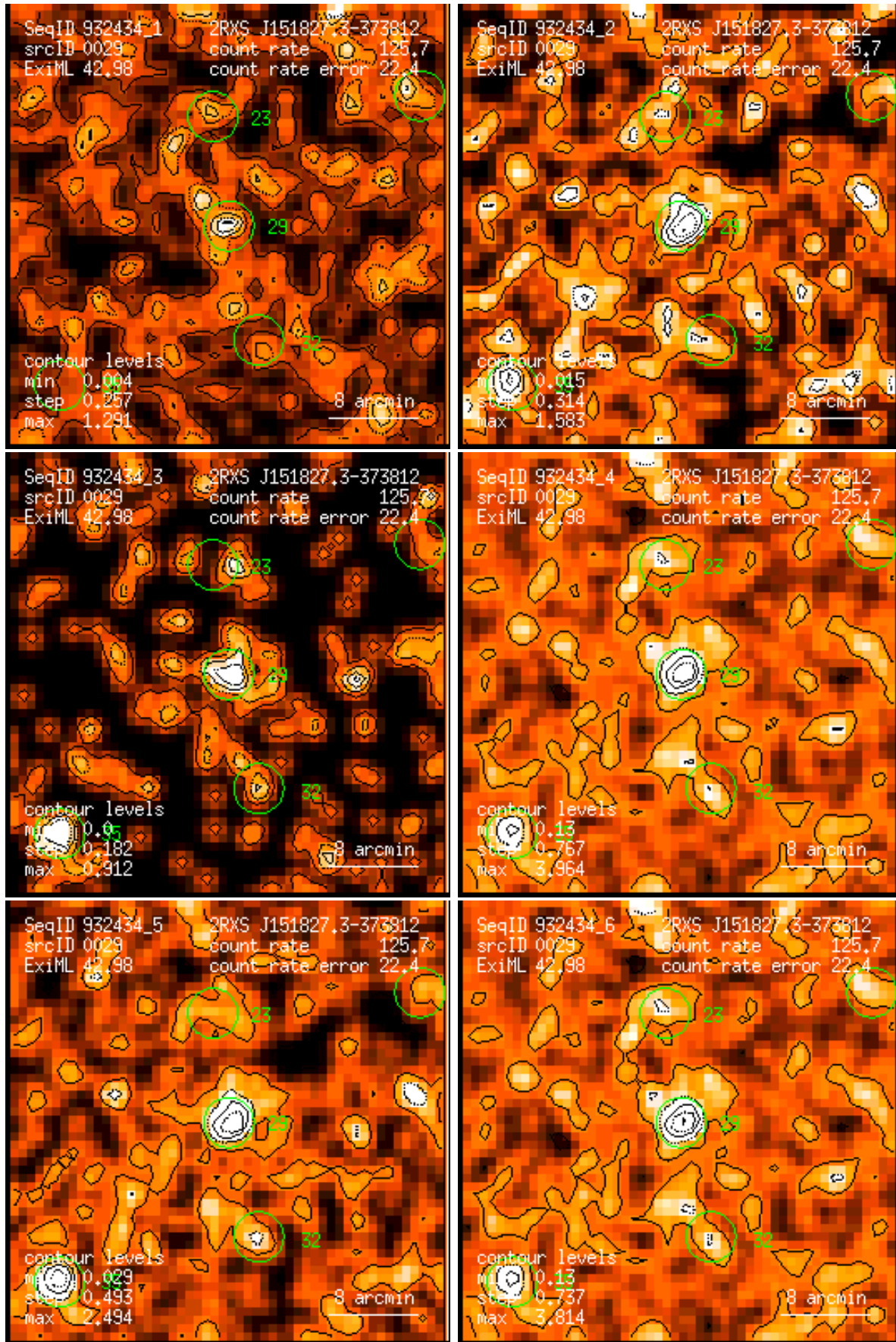
Figure 29: RASS 932434: detection 0029: band rate images, Gaussian filter: (1) PSPC channels 11 – 41, (2) 52 – 90, (3) 91 – 201, (4) 11 – 235, (5) 52 – 201, (6) 11 – 201. Broad band rates in counts/ks. Band rate contour levels in counts/ks/arcmin 2 .
