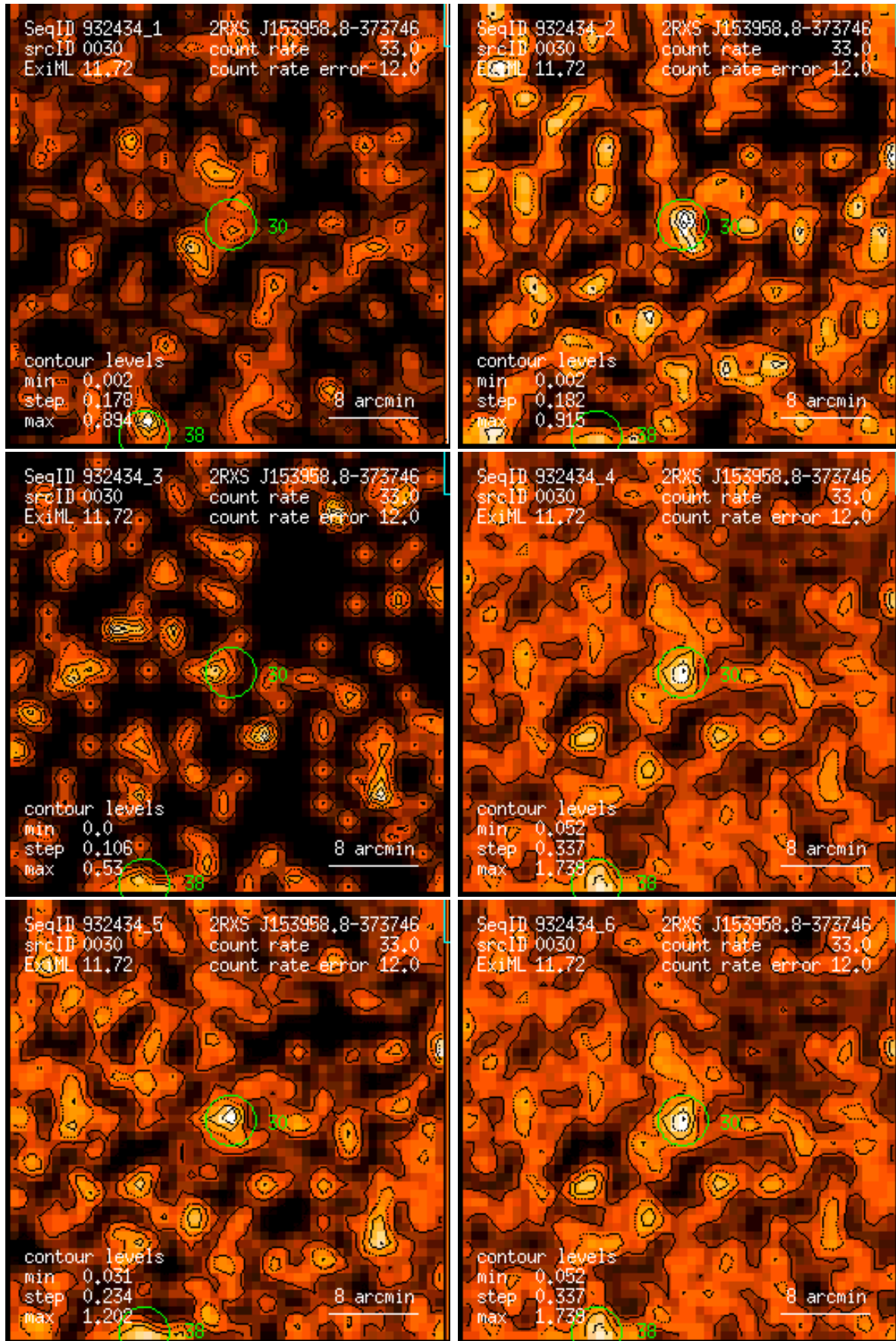
Figure 30: RASS 932434: detection 0030: band rate images, Gaussian filter: (1) PSPC channels 11 – 41, (2) 52 – 90, (3) 91 – 201, (4) 11 – 235, (5) 52 – 201, (6) 11 – 201. Broad band rates in counts/ks. Band rate contour levels in counts/ks/arcmin 2 .
