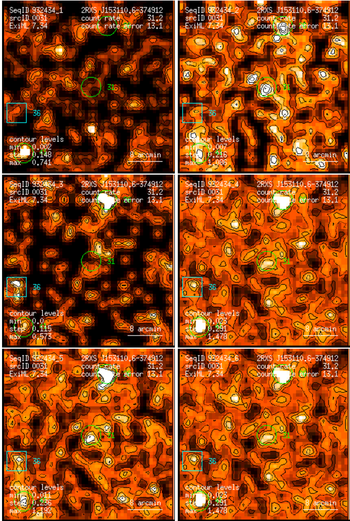
Figure 31: RASS 932434: detection 0031: band rate images, Gaussian filter: (1) PSPC channels 11 – 41, (2) 52 – 90, (3) 91 – 201, (4) 11 – 235, (5) 52 – 201, (6) 11 – 201. Broad band rates in counts/ks. Band rate contour levels in counts/ks/arcmin 2 .
