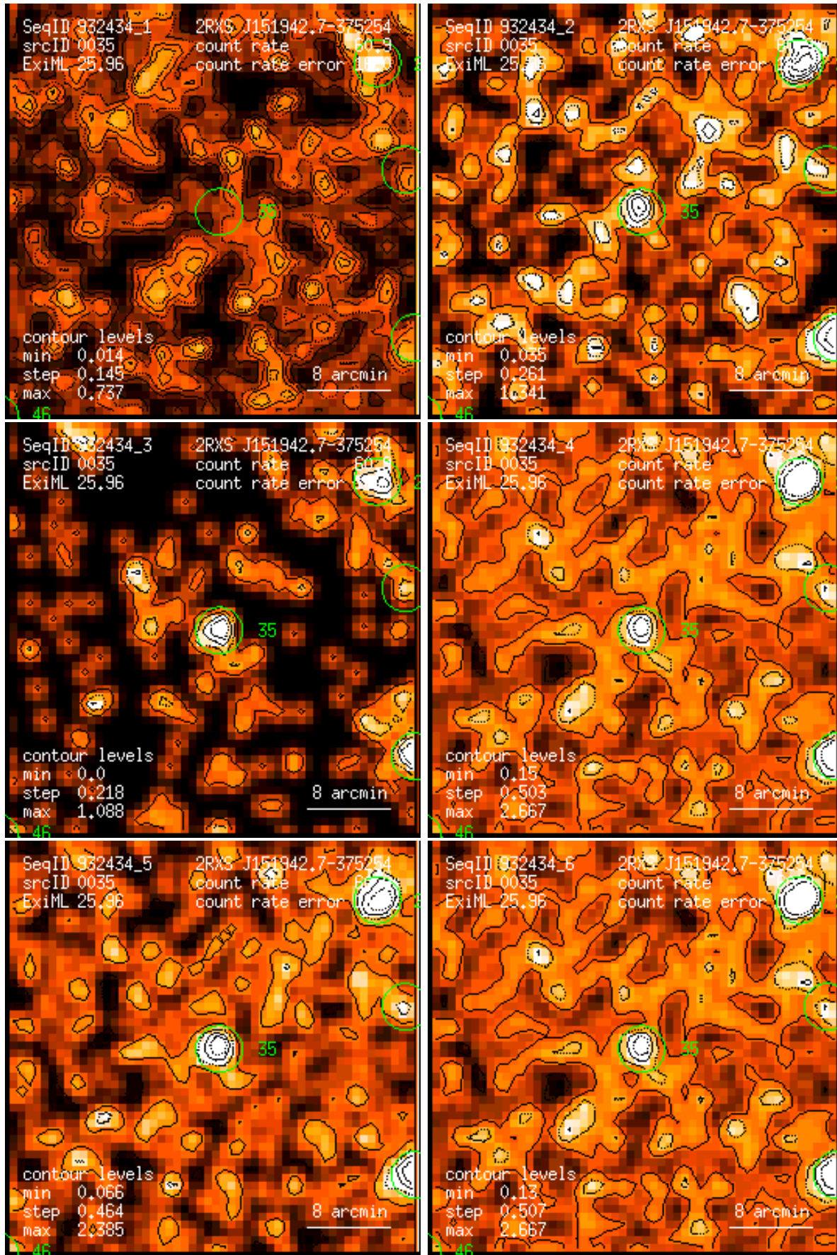
Figure 35: RASS 932434: detection 0035: band rate images, Gaussian filter: (1) PSPC channels 11 – 41, (2) 52 – 90, (3) 91 – 201, (4) 11 – 235, (5) 52 – 201, (6) 11 – 201. Broad band rates in counts/ks. Band rate contour levels in counts/ks/arcmin 2 .
