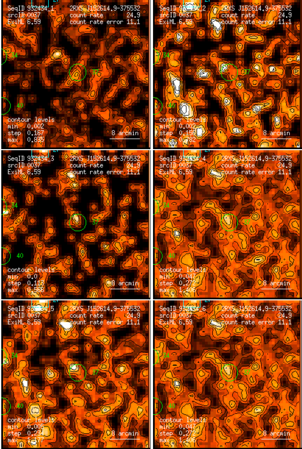
Figure 37: RASS 932434: detection 0037: band rate images, Gaussian filter: (1) PSPC channels 11 – 41, (2) 52 – 90, (3) 91 – 201, (4) 11 – 235, (5) 52 – 201, (6) 11 – 201. Broad band rates in counts/ks. Band rate contour levels in counts/ks/arcmin 2 .
