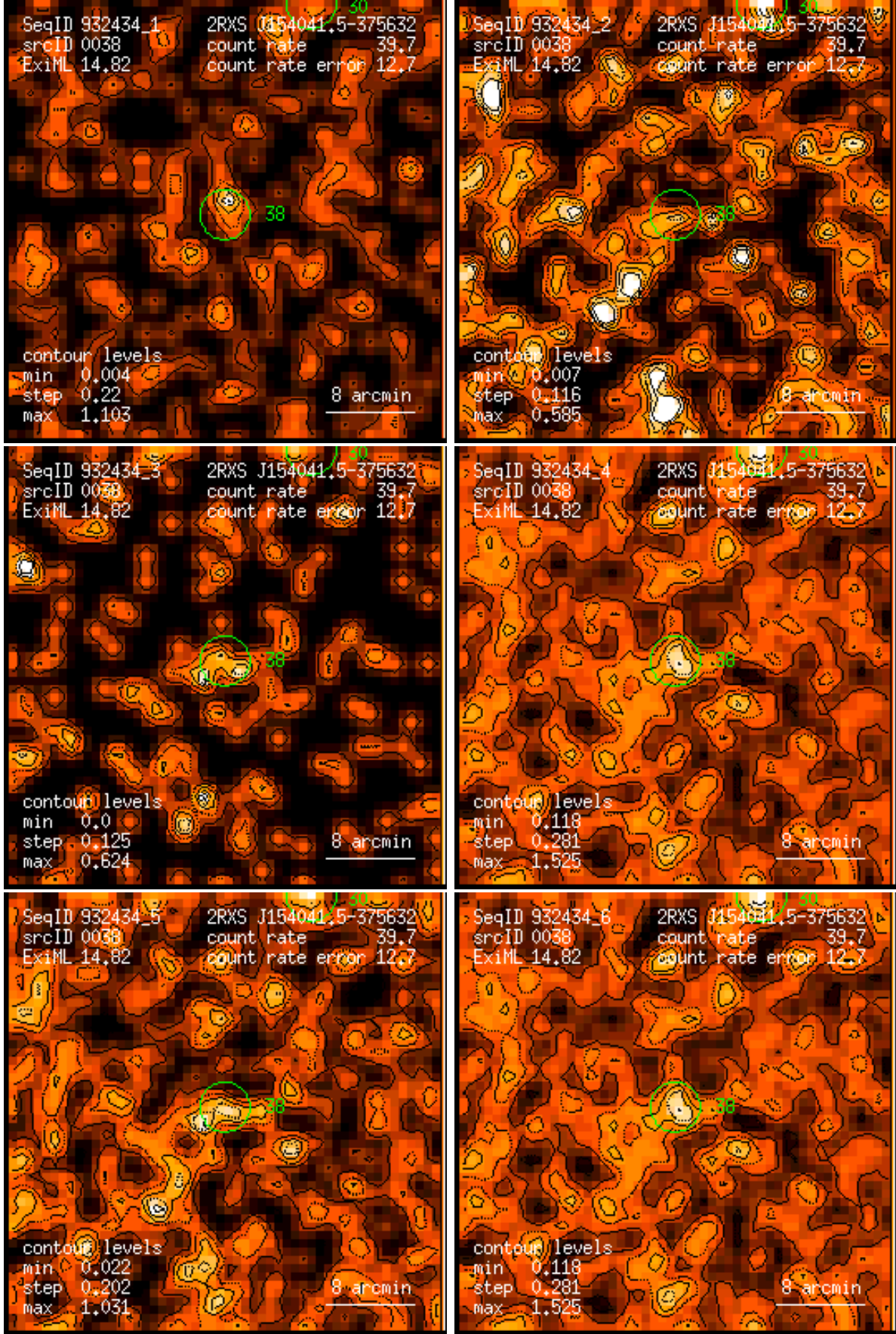
Figure 38: RASS 932434: detection 0038: band rate images, Gaussian filter: (1) PSPC channels 11 – 41, (2) 52 – 90, (3) 91 – 201, (4) 11 – 235, (5) 52 – 201, (6) 11 – 201. Broad band rates in counts/ks. Band rate contour levels in counts/ks/arcmin 2 .
