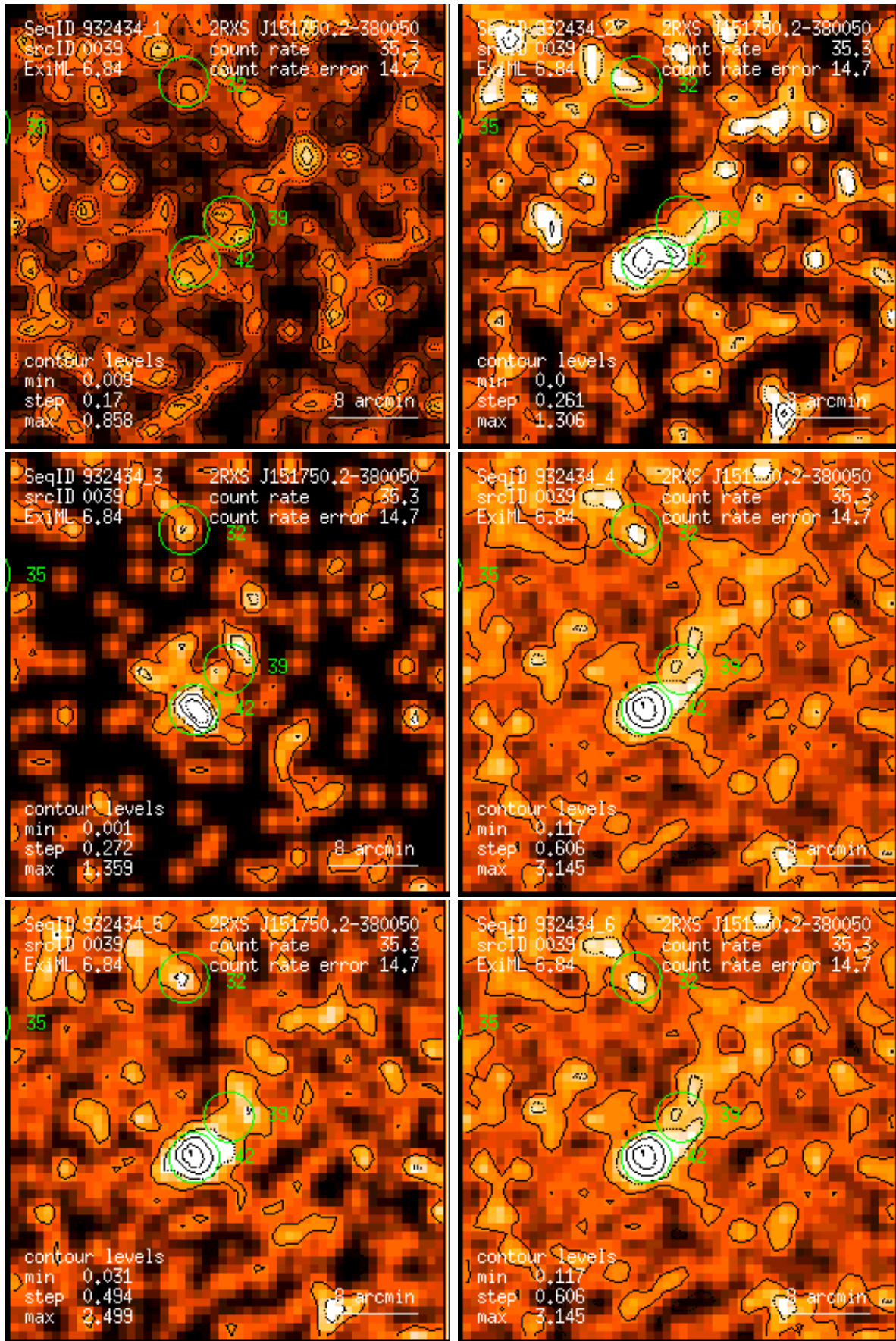
Figure 39: RASS 932434: detection 0039: band rate images, Gaussian filter: (1) PSPC channels 11 – 41, (2) 52 – 90, (3) 91 – 201, (4) 11 – 235, (5) 52 – 201, (6) 11 – 201. Broad band rates in counts/ks. Band rate contour levels in counts/ks/arcmin 2 .
