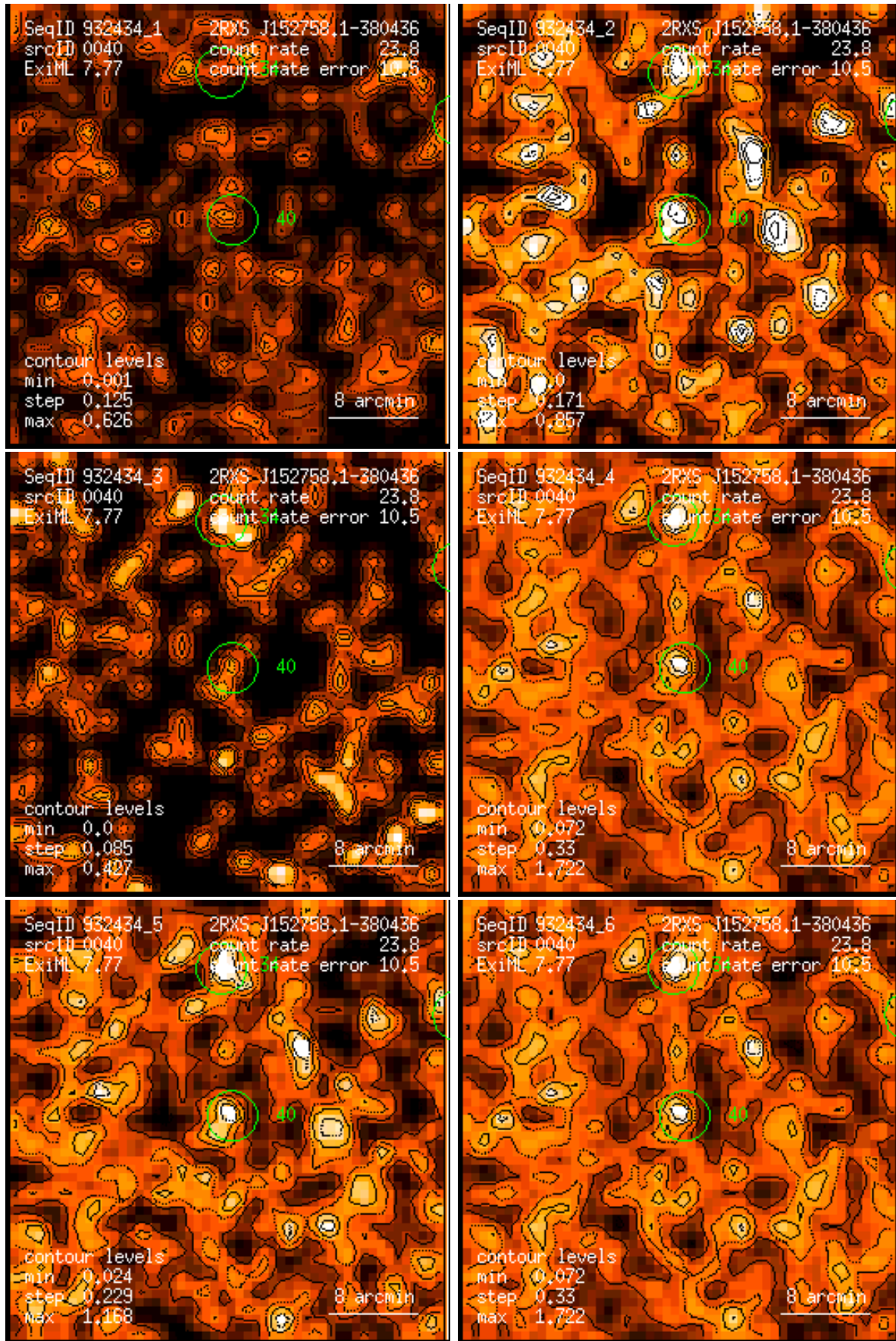
Figure 40: RASS 932434: detection 0040: band rate images, Gaussian filter: (1) PSPC channels 11 – 41, (2) 52 – 90, (3) 91 – 201, (4) 11 – 235, (5) 52 – 201, (6) 11 – 201. Broad band rates in counts/ks. Band rate contour levels in counts/ks/arcmin 2 .
