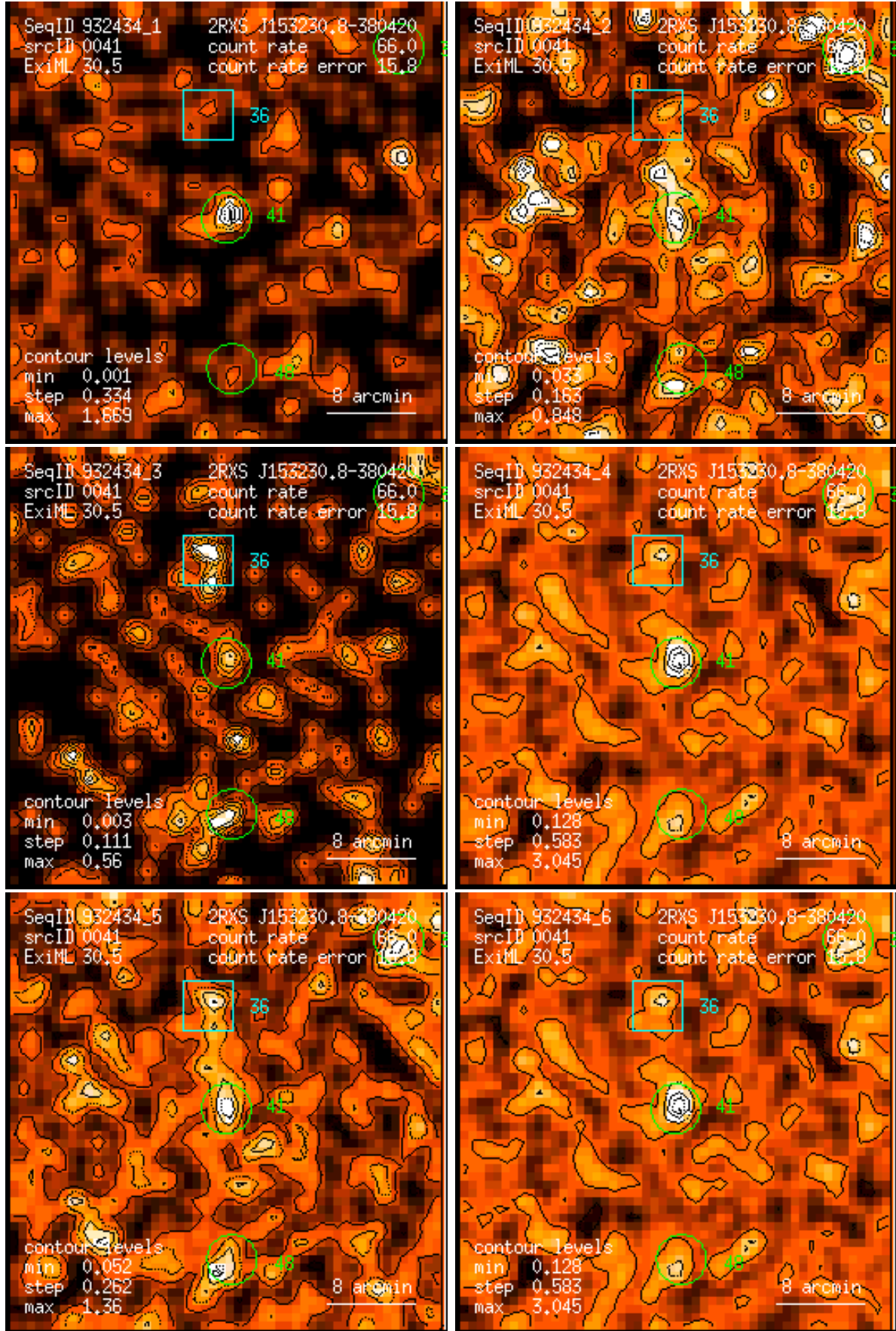
Figure 41: RASS 932434: detection 0041: band rate images, Gaussian filter: (1) PSPC channels 11 – 41, (2) 52 – 90, (3) 91 – 201, (4) 11 – 235, (5) 52 – 201, (6) 11 – 201. Broad band rates in counts/ks. Band rate contour levels in counts/ks/arcmin 2 .
