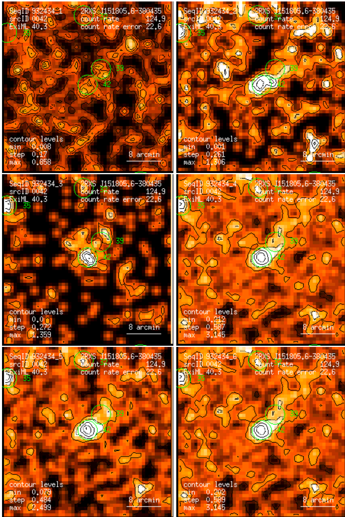
Figure 42: RASS 932434: detection 0042: band rate images, Gaussian filter: (1) PSPC channels 11 – 41, (2) 52 – 90, (3) 91 – 201, (4) 11 – 235, (5) 52 – 201, (6) 11 – 201. Broad band rates in counts/ks. Band rate contour levels in counts/ks/arcmin 2 .
