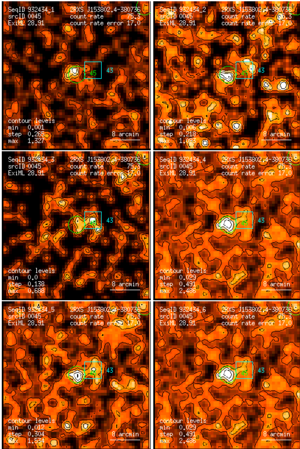
Figure 45: RASS 932434: detection 0045: band rate images, Gaussian filter: (1) PSPC channels 11 – 41, (2) 52 – 90, (3) 91 – 201, (4) 11 – 235, (5) 52 – 201, (6) 11 – 201. Broad band rates in counts/ks. Band rate contour levels in counts/ks/arcmin 2 .
