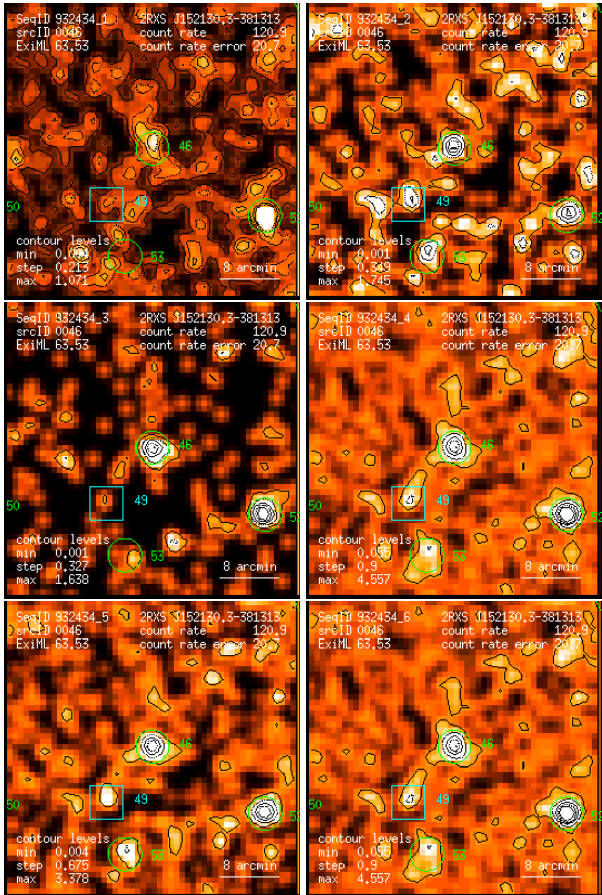
Figure 46: RASS 932434: detection 0046: band rate images, Gaussian filter: (1) PSPC channels 11 – 41, (2) 52 – 90, (3) 91 – 201, (4) 11 – 235, (5) 52 – 201, (6) 11 – 201. Broad band rates in counts/ks. Band rate contour levels in counts/ks/arcmin 2 .
