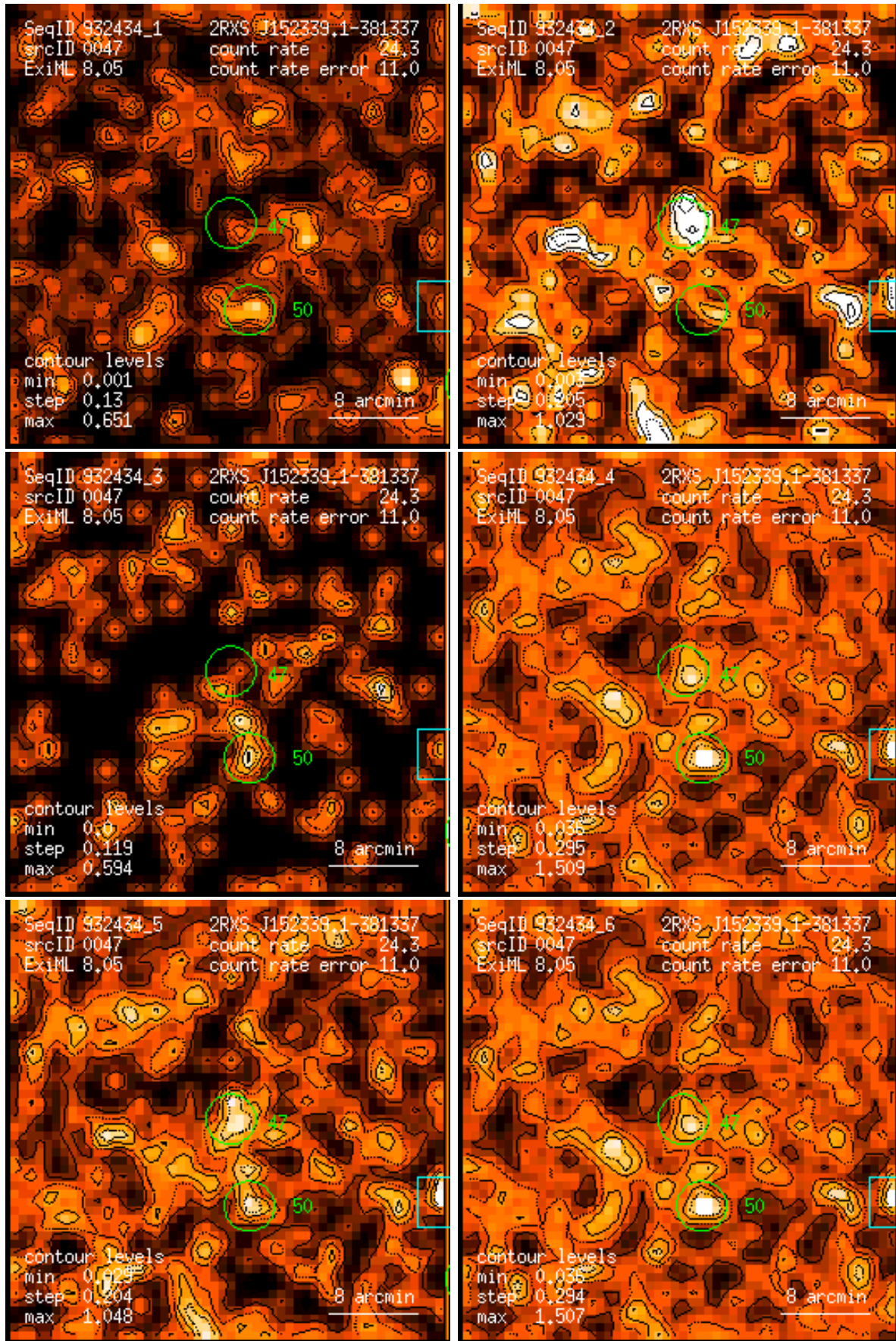
Figure 47: RASS 932434: detection 0047: band rate images, Gaussian filter: (1) PSPC channels 11 – 41, (2) 52 – 90, (3) 91 – 201, (4) 11 – 235, (5) 52 – 201, (6) 11 – 201. Broad band rates in counts/ks. Band rate contour levels in counts/ks/arcmin 2 .
