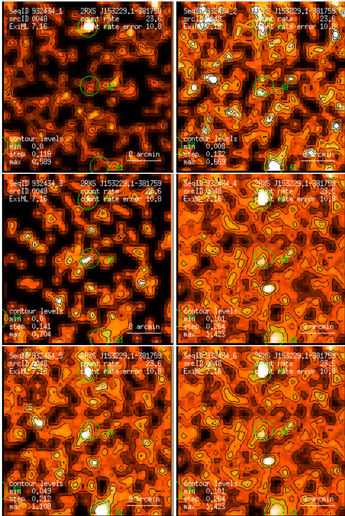
Figure 48: RASS 932434: detection 0048: band rate images, Gaussian filter: (1) PSPC channels 11 – 41, (2) 52 – 90, (3) 91 – 201, (4) 11 – 235, (5) 52 – 201, (6) 11 – 201. Broad band rates in counts/ks. Band rate contour levels in counts/ks/arcmin 2 .
