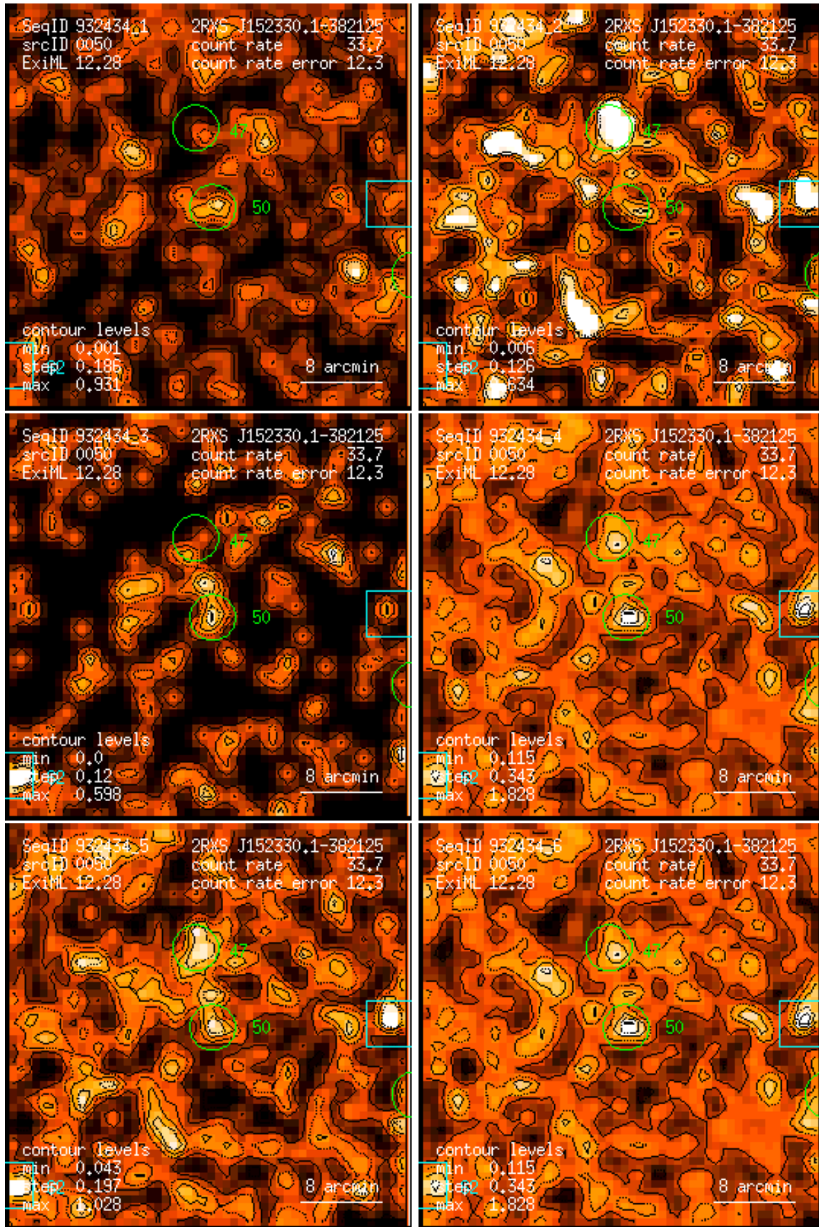
Figure 50: RASS 932434: detection 0050: band rate images, Gaussian filter: (1) PSPC channels 11 – 41, (2) 52 – 90, (3) 91 – 201, (4) 11 – 235, (5) 52 – 201, (6) 11 – 201. Broad band rates in counts/ks. Band rate contour levels in counts/ks/arcmin 2 .
