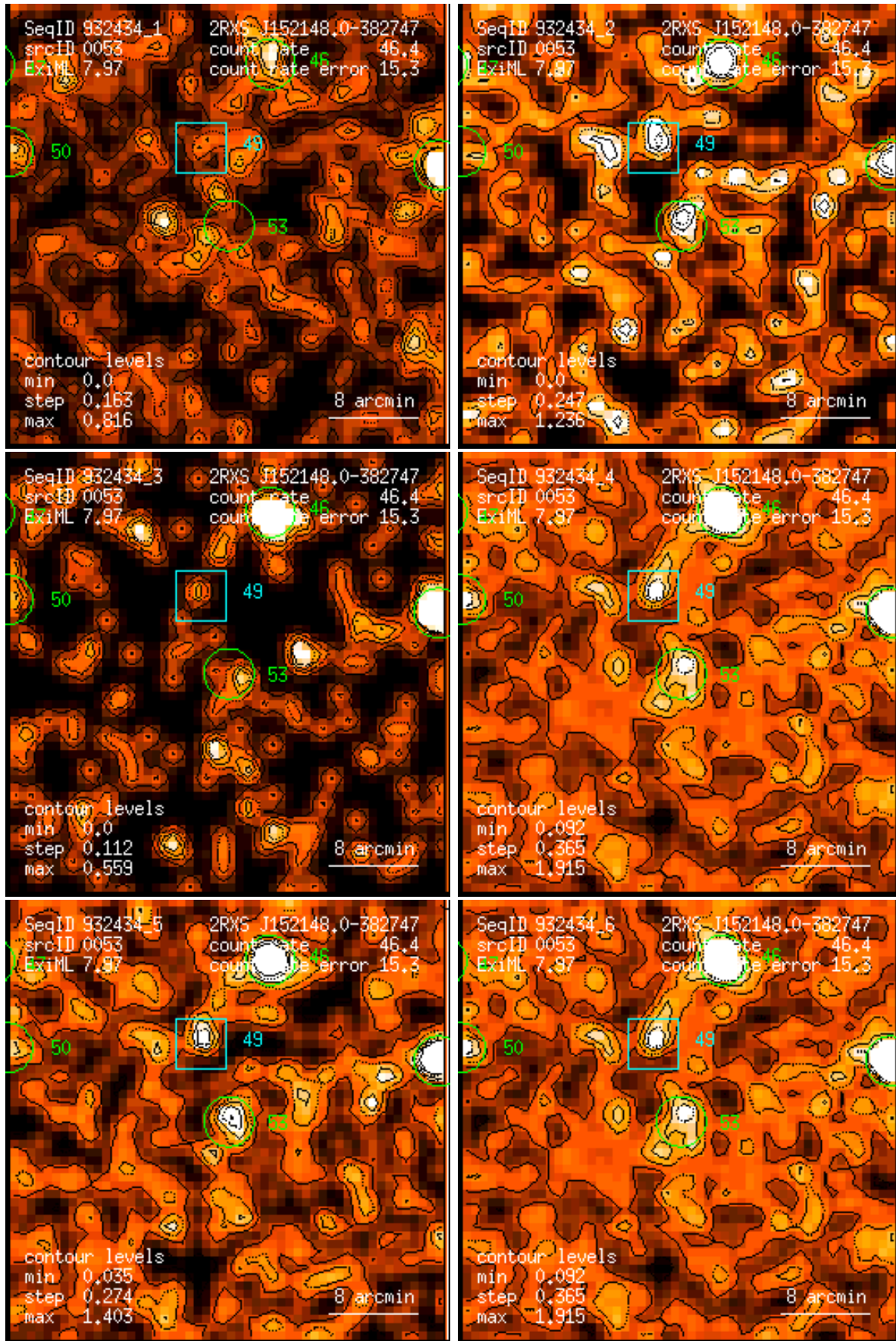
Figure 53: RASS 932434: detection 0053: band rate images, Gaussian filter: (1) PSPC channels 11 – 41, (2) 52 – 90, (3) 91 – 201, (4) 11 – 235, (5) 52 – 201, (6) 11 – 201. Broad band rates in counts/ks. Band rate contour levels in counts/ks/arcmin 2 .
