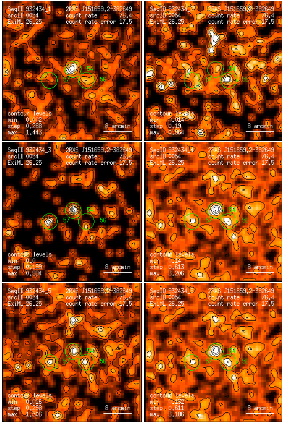
Figure 54: RASS 932434: detection 0054: band rate images, Gaussian filter: (1) PSPC channels 11 – 41, (2) 52 – 90, (3) 91 – 201, (4) 11 – 235, (5) 52 – 201, (6) 11 – 201. Broad band rates in counts/ks. Band rate contour levels in counts/ks/arcmin 2 .
