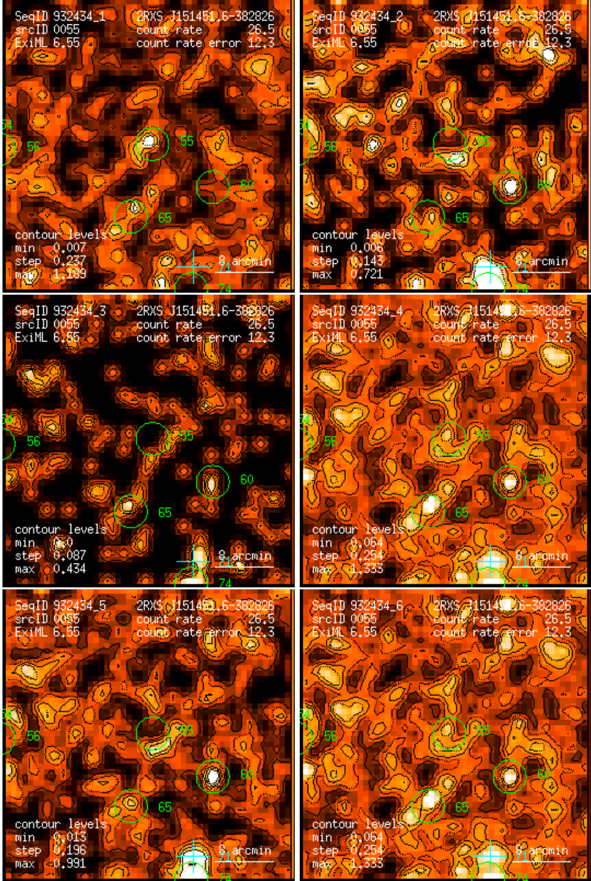
Figure 55: RASS 932434: detection 0055: band rate images, Gaussian filter: (1) PSPC channels 11 – 41, (2) 52 – 90, (3) 91 – 201, (4) 11 – 235, (5) 52 – 201, (6) 11 – 201. Broad band rates in counts/ks. Band rate contour levels in counts/ks/arcmin 2 .
