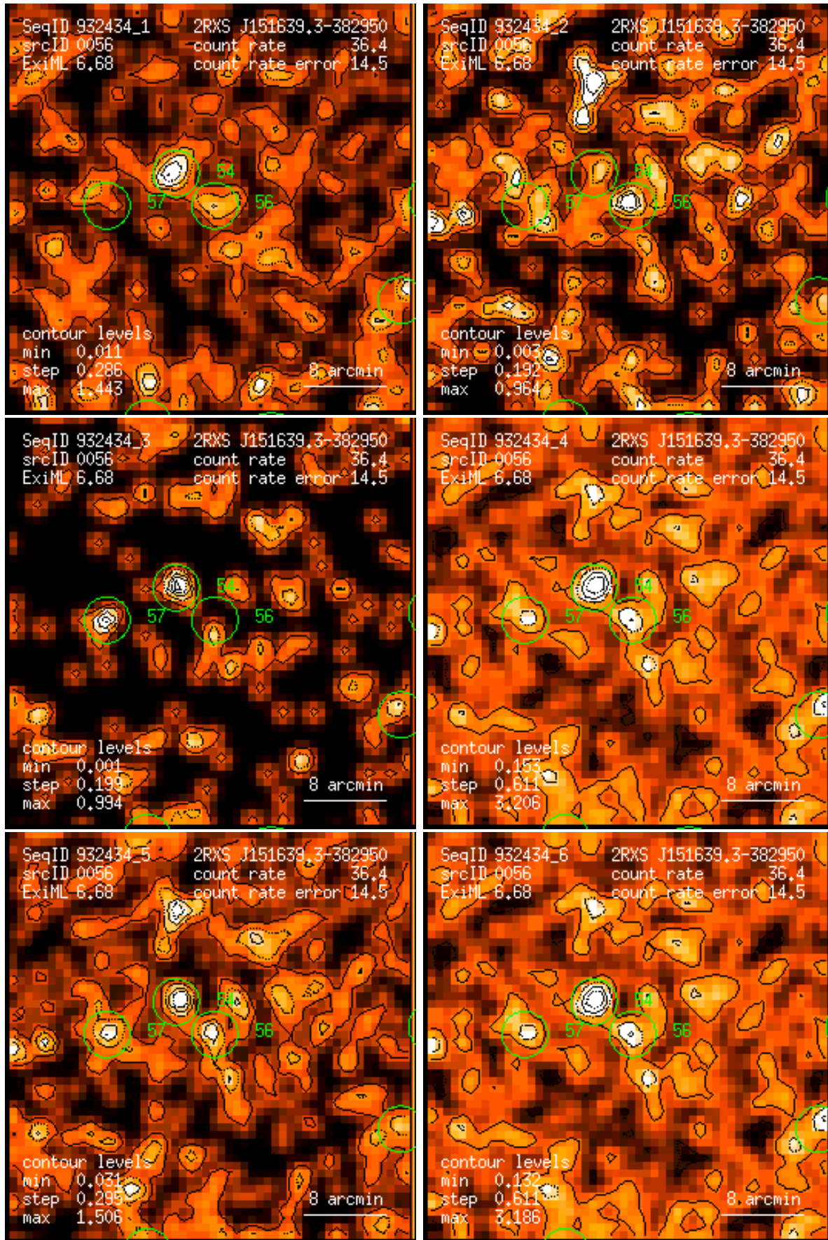
Figure 56: RASS 932434: detection 0056: band rate images, Gaussian filter: (1) PSPC channels 11 – 41, (2) 52 – 90, (3) 91 – 201, (4) 11 – 235, (5) 52 – 201, (6) 11 – 201. Broad band rates in counts/ks. Band rate contour levels in counts/ks/arcmin 2 .
