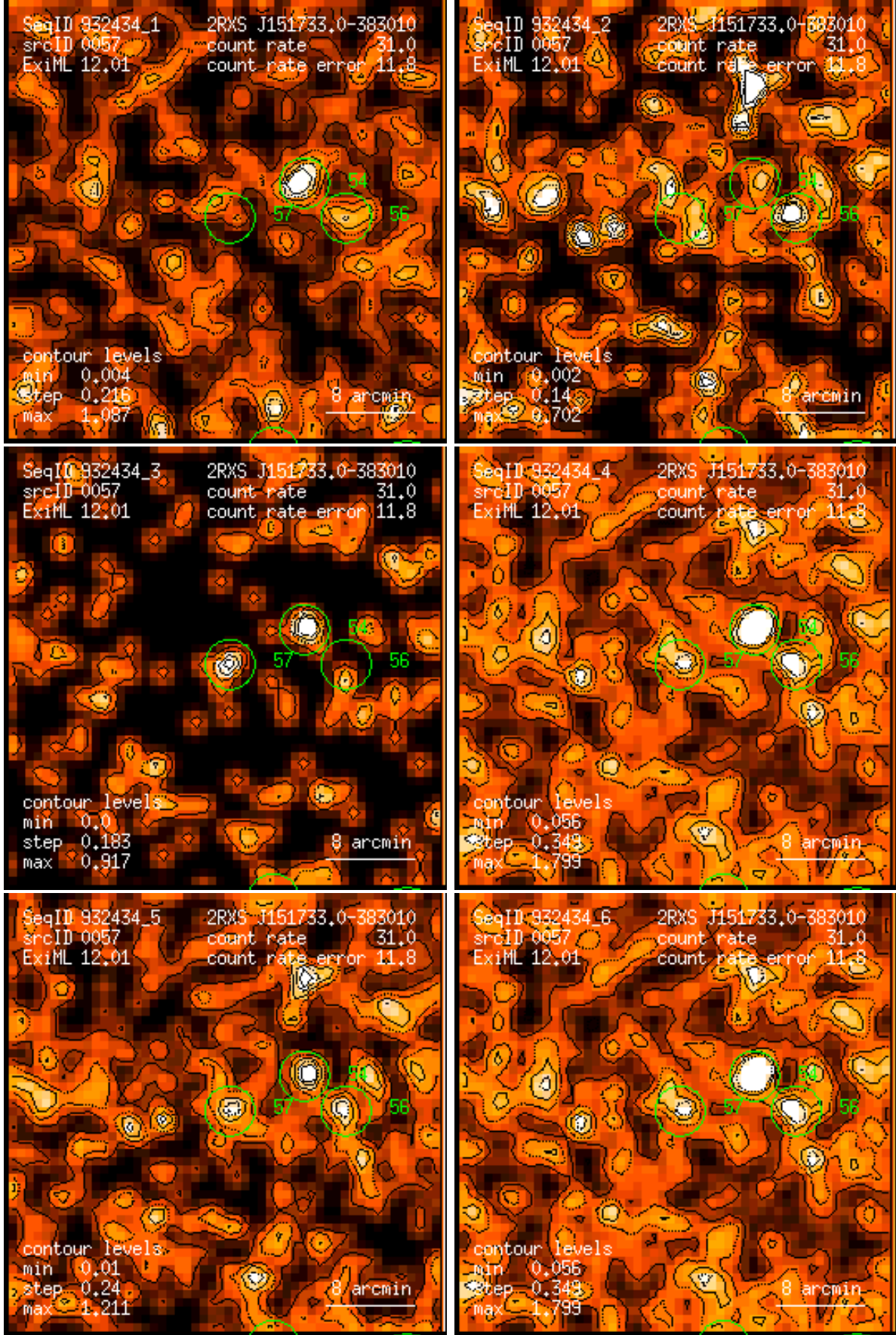
Figure 57: RASS 932434: detection 0057: band rate images, Gaussian filter: (1) PSPC channels 11 – 41, (2) 52 – 90, (3) 91 – 201, (4) 11 – 235, (5) 52 – 201, (6) 11 – 201. Broad band rates in counts/ks. Band rate contour levels in counts/ks/arcmin 2 .
