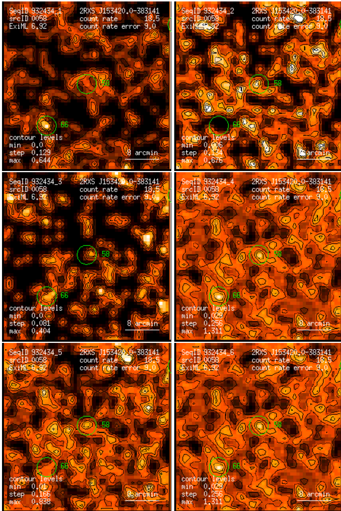
Figure 58: RASS 932434: detection 0058: band rate images, Gaussian filter: (1) PSPC channels 11 – 41, (2) 52 – 90, (3) 91 – 201, (4) 11 – 235, (5) 52 – 201, (6) 11 – 201. Broad band rates in counts/ks. Band rate contour levels in counts/ks/arcmin 2 .
