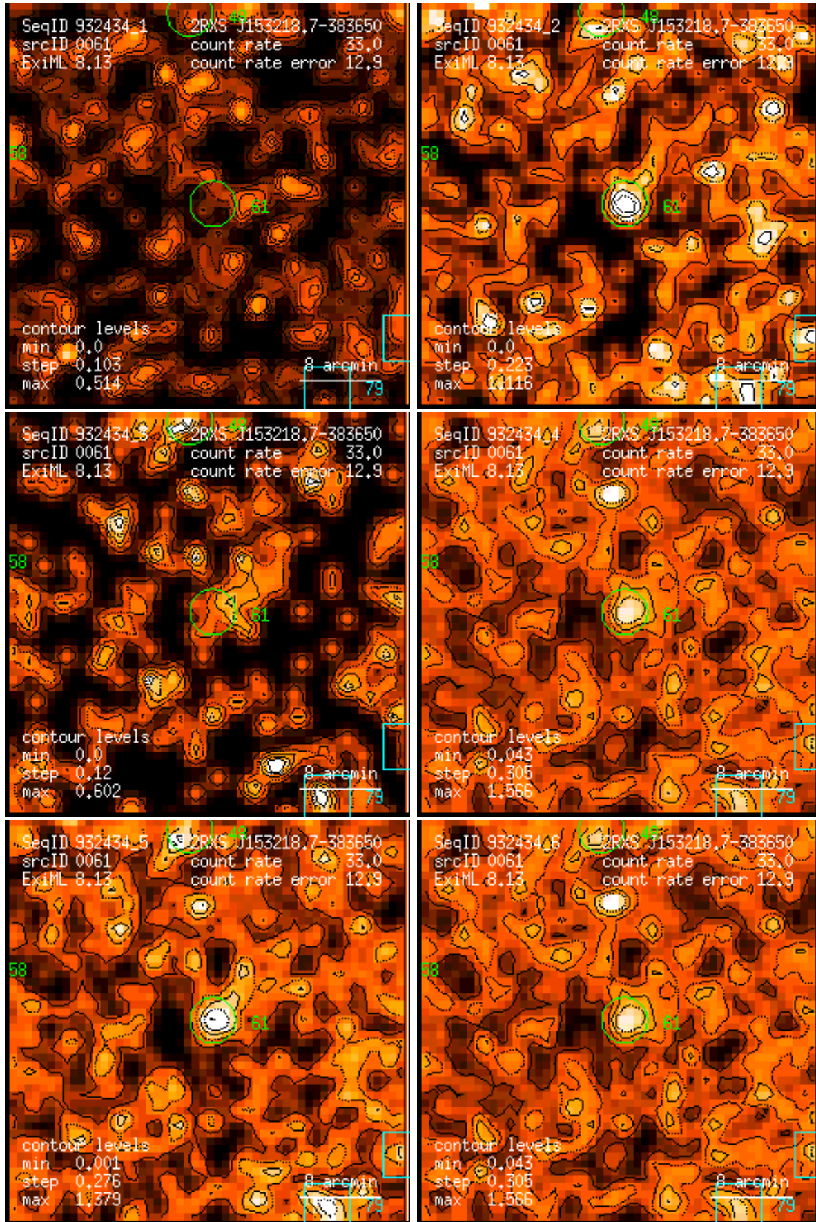
Figure 61: RASS 932434: detection 0061: band rate images, Gaussian filter: (1) PSPC channels 11 – 41, (2) 52 – 90, (3) 91 – 201, (4) 11 – 235, (5) 52 – 201, (6) 11 – 201. Broad band rates in counts/ks. Band rate contour levels in counts/ks/arcmin 2 .
