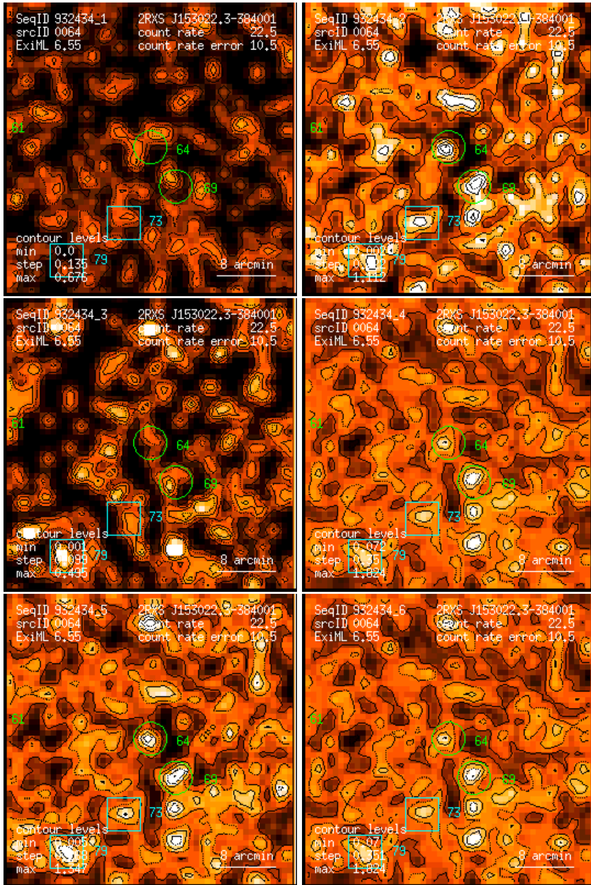
Figure 64: RASS 932434: detection 0064: band rate images, Gaussian filter: (1) PSPC channels 11 – 41, (2) 52 – 90, (3) 91 – 201, (4) 11 – 235, (5) 52 – 201, (6) 11 – 201. Broad band rates in counts/ks. Band rate contour levels in counts/ks/arcmin 2 .
