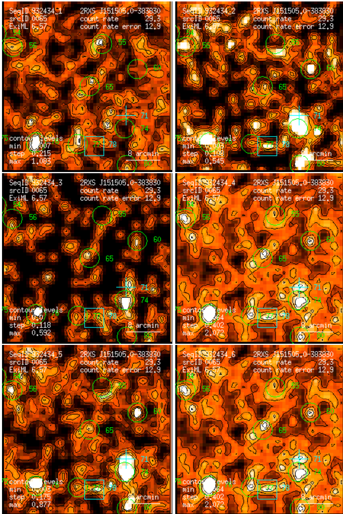
Figure 65: RASS 932434: detection 0065: band rate images, Gaussian filter: (1) PSPC channels 11 – 41, (2) 52 – 90, (3) 91 – 201, (4) 11 – 235, (5) 52 – 201, (6) 11 – 201. Broad band rates in counts/ks. Band rate contour levels in counts/ks/arcmin 2 .
