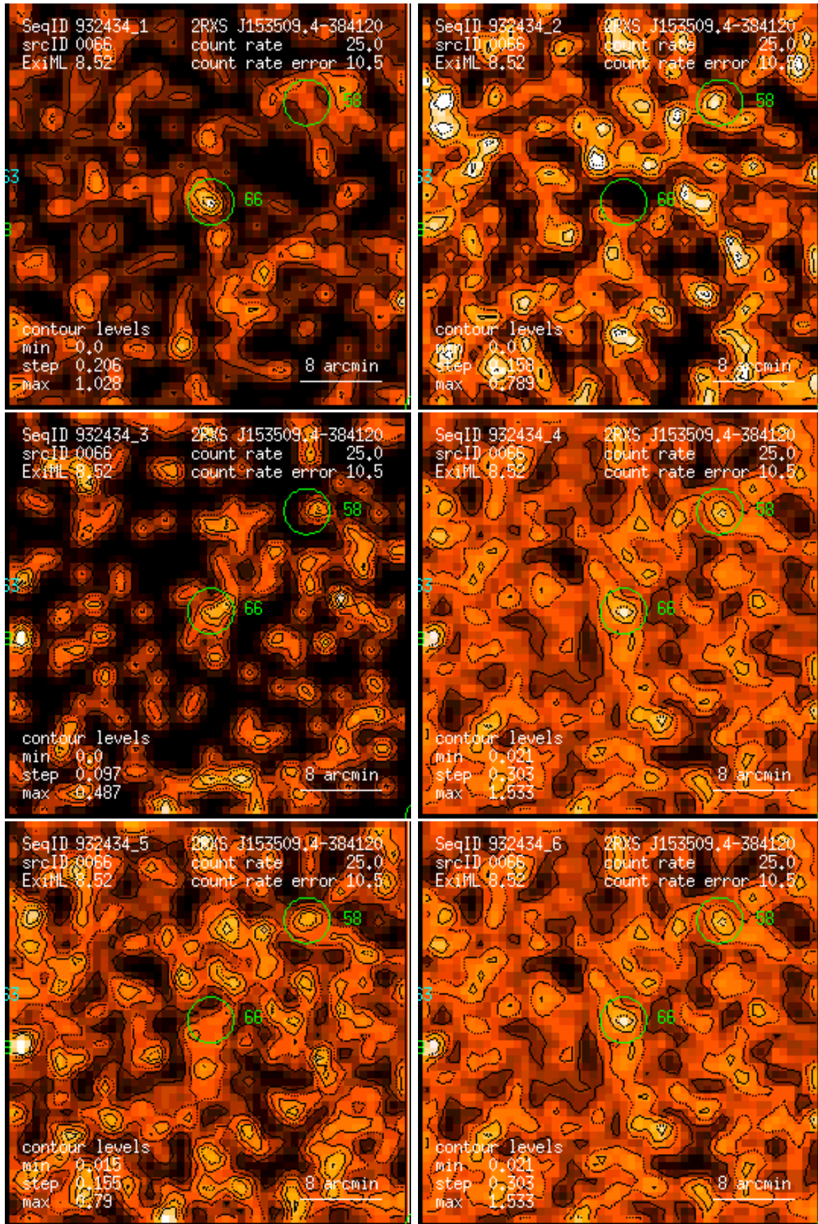
Figure 66: RASS 932434: detection 0066: band rate images, Gaussian filter: (1) PSPC channels 11 – 41, (2) 52 – 90, (3) 91 – 201, (4) 11 – 235, (5) 52 – 201, (6) 11 – 201. Broad band rates in counts/ks. Band rate contour levels in counts/ks/arcmin 2 .
