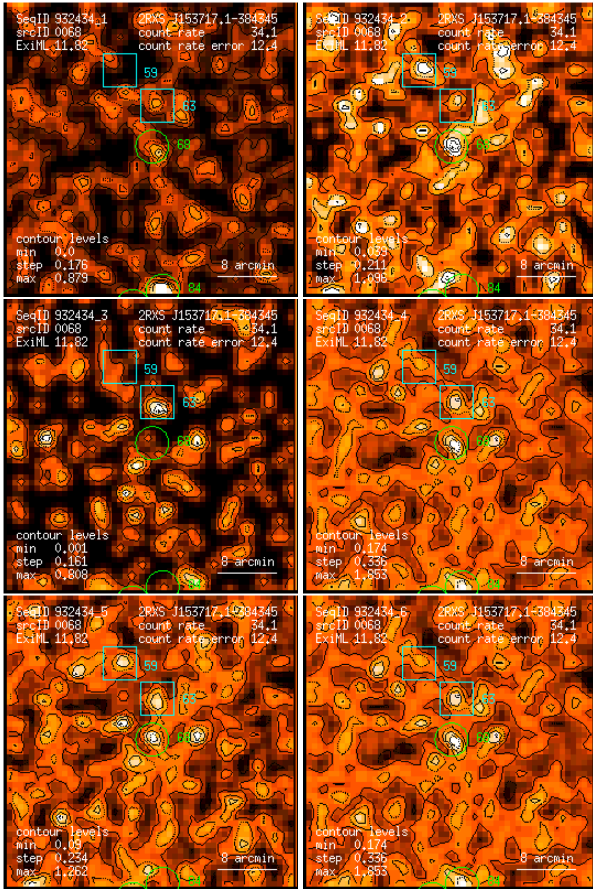
Figure 68: RASS 932434: detection 0068: band rate images, Gaussian filter: (1) PSPC channels 11 – 41, (2) 52 – 90, (3) 91 – 201, (4) 11 – 235, (5) 52 – 201, (6) 11 – 201. Broad band rates in counts/ks. Band rate contour levels in counts/ks/arcmin 2 .
