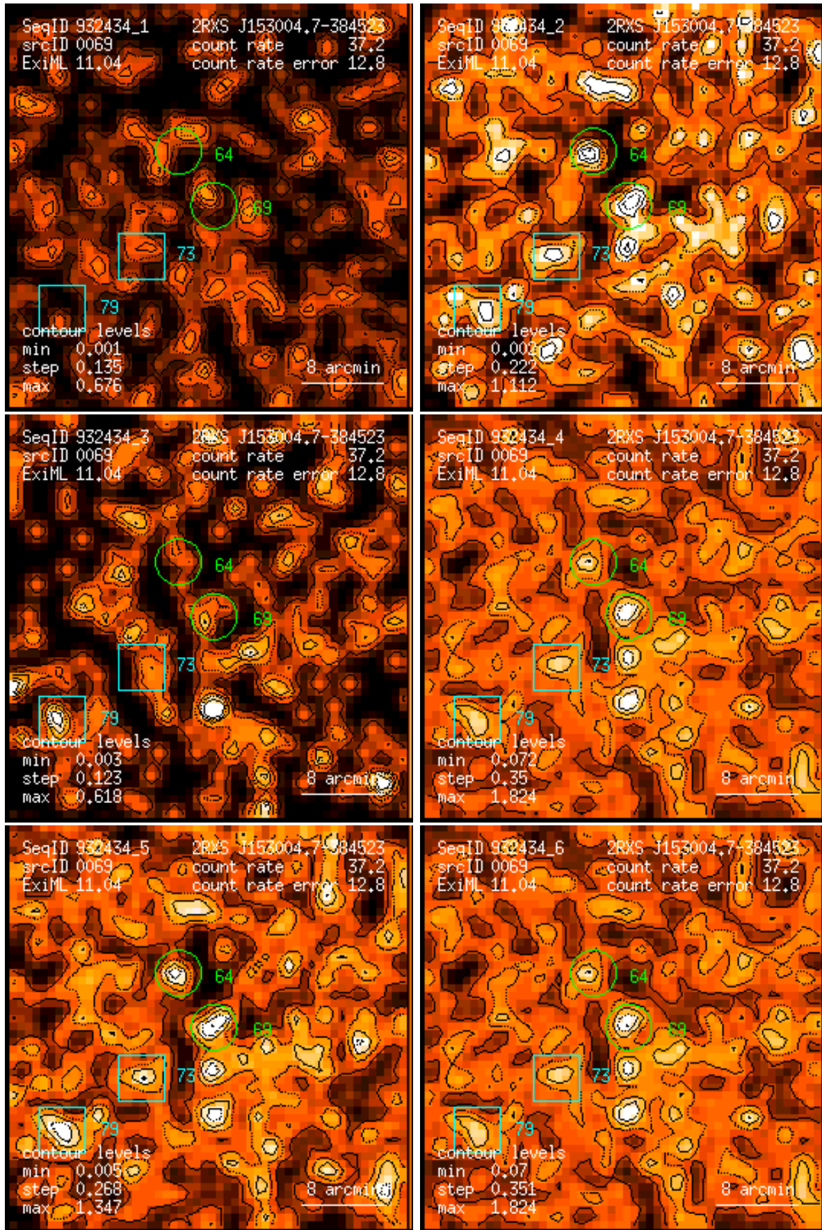
Figure 69: RASS 932434: detection 0069: band rate images, Gaussian filter: (1) PSPC channels 11 – 41, (2) 52 – 90, (3) 91 – 201, (4) 11 – 235, (5) 52 – 201, (6) 11 – 201. Broad band rates in counts/ks. Band rate contour levels in counts/ks/arcmin 2 .
