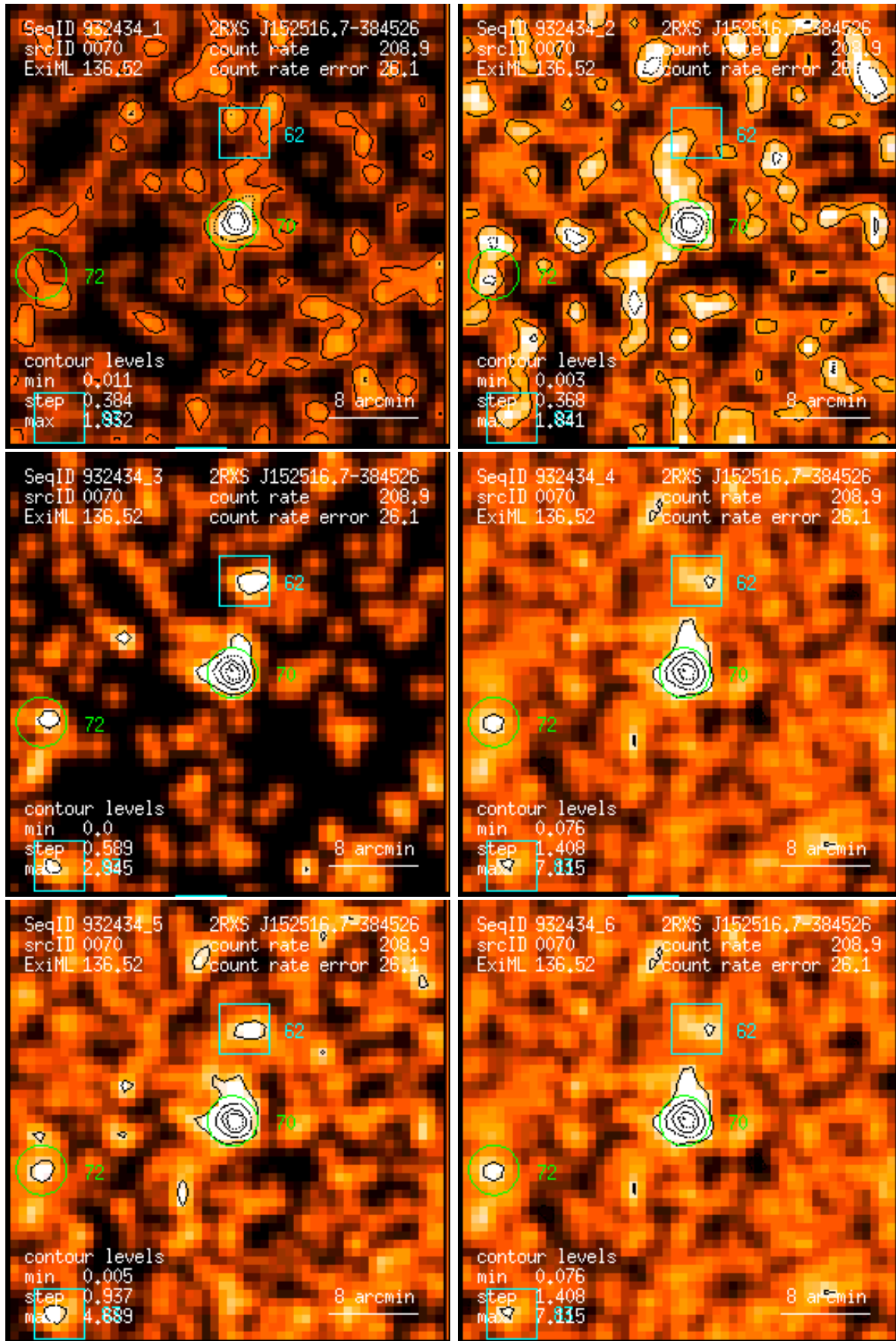
Figure 70: RASS 932434: detection 0070: band rate images, Gaussian filter: (1) PSPC channels 11 – 41, (2) 52 – 90, (3) 91 – 201, (4) 11 – 235, (5) 52 – 201, (6) 11 – 201. Broad band rates in counts/ks. Band rate contour levels in counts/ks/arcmin 2 .
