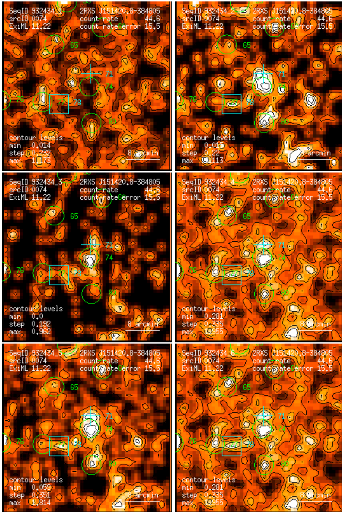
Figure 74: RASS 932434: detection 0074: band rate images, Gaussian filter: (1) PSPC channels 11 – 41, (2) 52 – 90, (3) 91 – 201, (4) 11 – 235, (5) 52 – 201, (6) 11 – 201. Broad band rates in counts/ks. Band rate contour levels in counts/ks/arcmin 2 .
