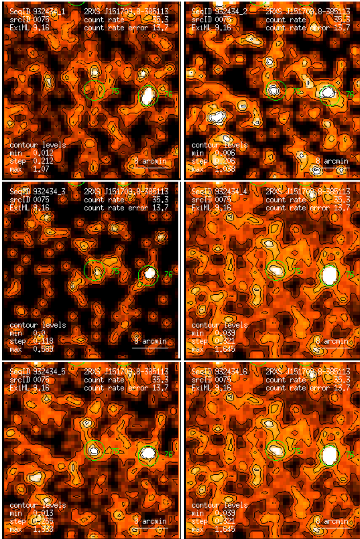
Figure 75: RASS 932434: detection 0075: band rate images, Gaussian filter: (1) PSPC channels 11 – 41, (2) 52 – 90, (3) 91 – 201, (4) 11 – 235, (5) 52 – 201, (6) 11 – 201. Broad band rates in counts/ks. Band rate contour levels in counts/ks/arcmin 2 .
