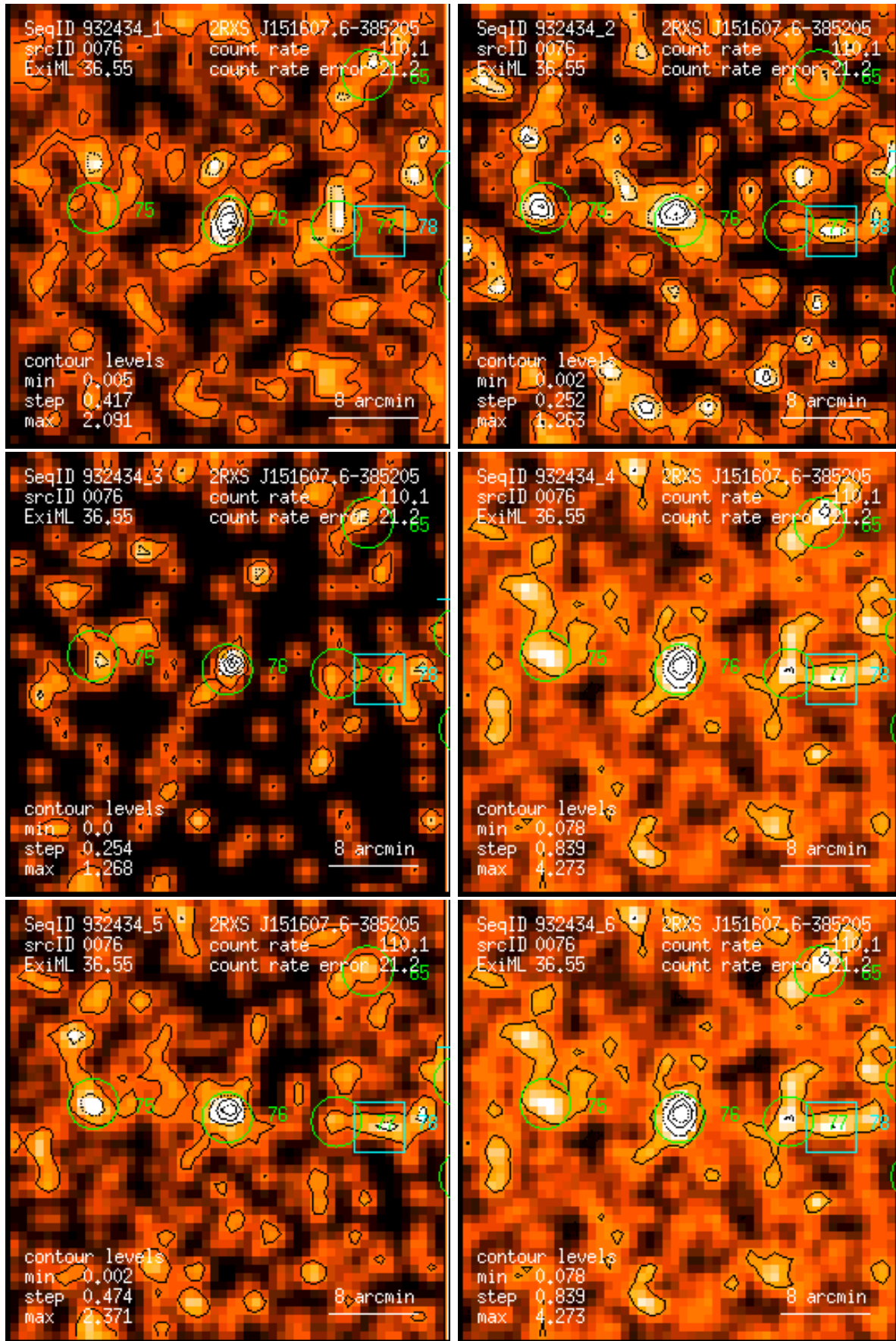
Figure 76: RASS 932434: detection 0076: band rate images, Gaussian filter: (1) PSPC channels 11 – 41, (2) 52 – 90, (3) 91 – 201, (4) 11 – 235, (5) 52 – 201, (6) 11 – 201. Broad band rates in counts/ks. Band rate contour levels in counts/ks/arcmin 2 .
