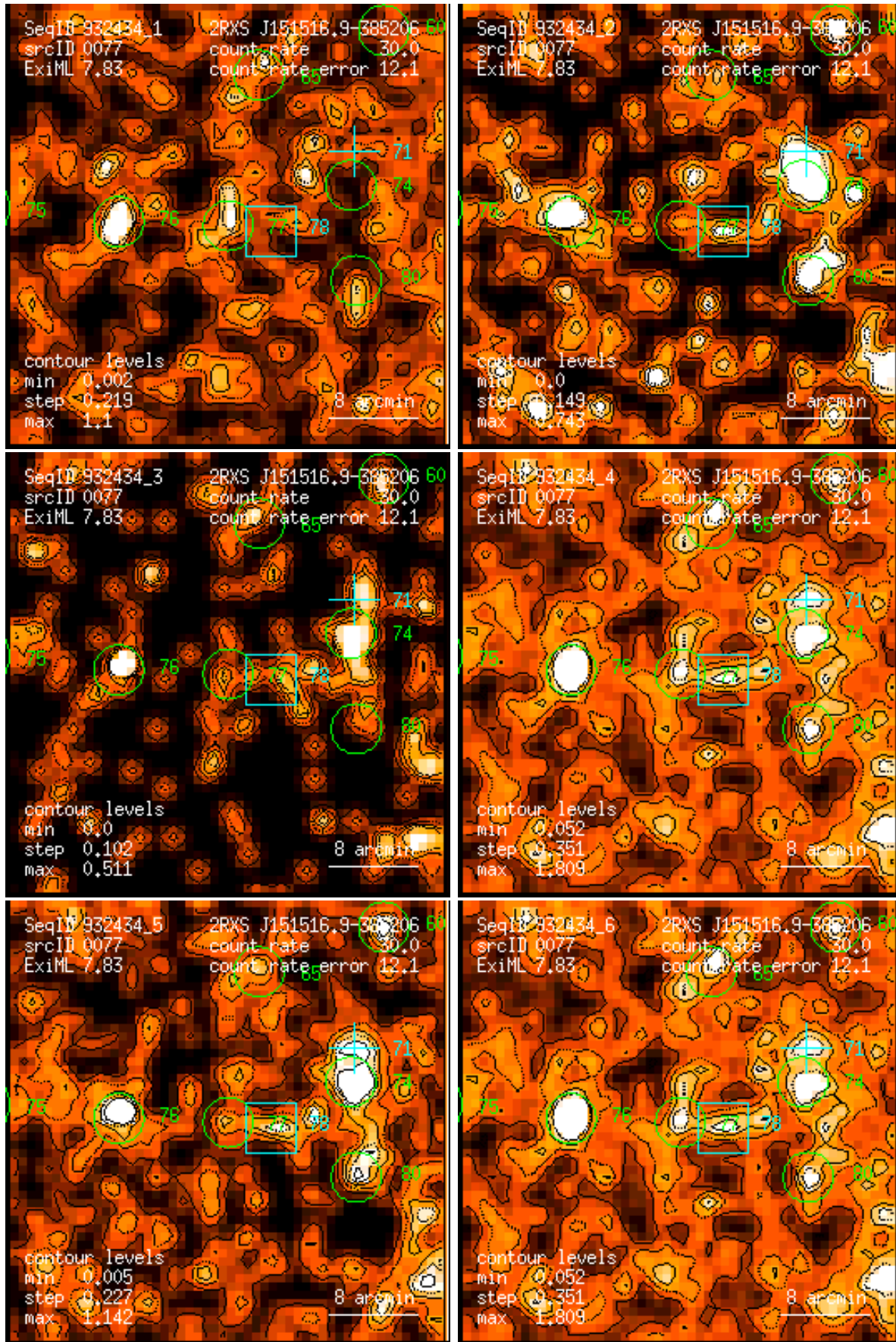
Figure 77: RASS 932434: detection 0077: band rate images, Gaussian filter: (1) PSPC channels 11 – 41, (2) 52 – 90, (3) 91 – 201, (4) 11 – 235, (5) 52 – 201, (6) 11 – 201. Broad band rates in counts/ks. Band rate contour levels in counts/ks/arcmin 2 .
