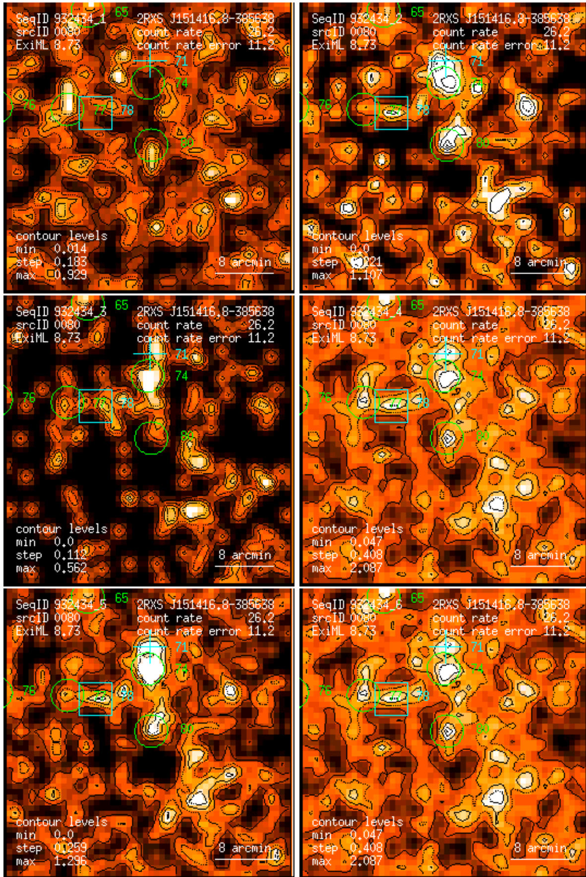
Figure 80: RASS 932434: detection 0080: band rate images, Gaussian filter: (1) PSPC channels 11 – 41, (2) 52 – 90, (3) 91 – 201, (4) 11 – 235, (5) 52 – 201, (6) 11 – 201. Broad band rates in counts/ks. Band rate contour levels in counts/ks/arcmin 2 .
