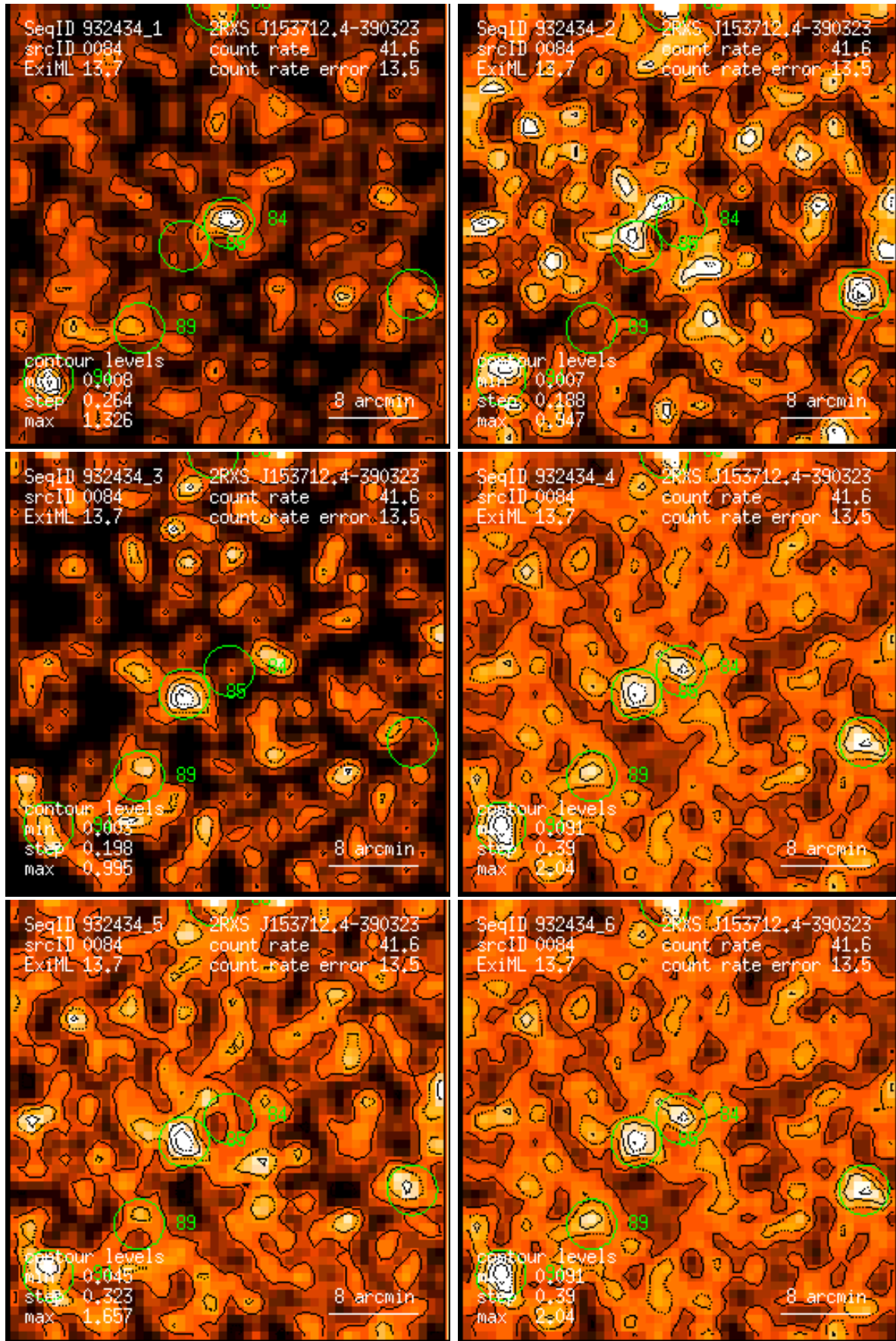
Figure 84: RASS 932434: detection 0084: band rate images, Gaussian filter: (1) PSPC channels 11 – 41, (2) 52 – 90, (3) 91 – 201, (4) 11 – 235, (5) 52 – 201, (6) 11 – 201. Broad band rates in counts/ks. Band rate contour levels in counts/ks/arcmin 2 .
