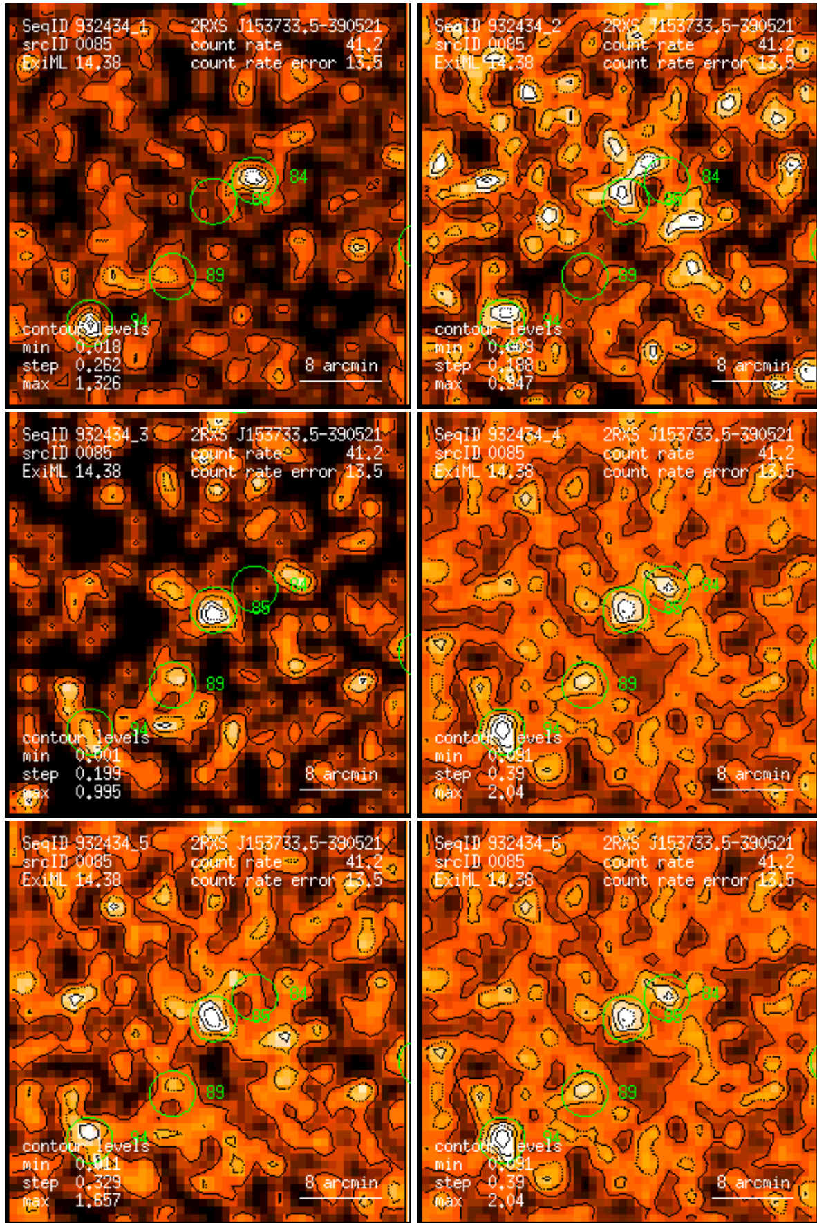
Figure 85: RASS 932434: detection 0085: band rate images, Gaussian filter: (1) PSPC channels 11 – 41, (2) 52 – 90, (3) 91 – 201, (4) 11 – 235, (5) 52 – 201, (6) 11 – 201. Broad band rates in counts/ks. Band rate contour levels in counts/ks/arcmin 2 .
