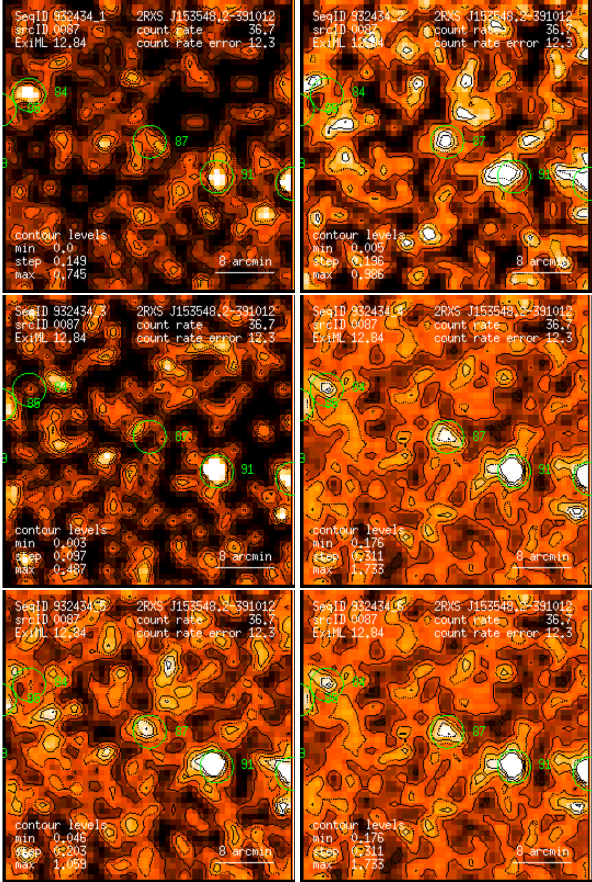
Figure 87: RASS 932434: detection 0087: band rate images, Gaussian filter: (1) PSPC channels 11 – 41, (2) 52 – 90, (3) 91 – 201, (4) 11 – 235, (5) 52 – 201, (6) 11 – 201. Broad band rates in counts/ks. Band rate contour levels in counts/ks/arcmin 2 .
