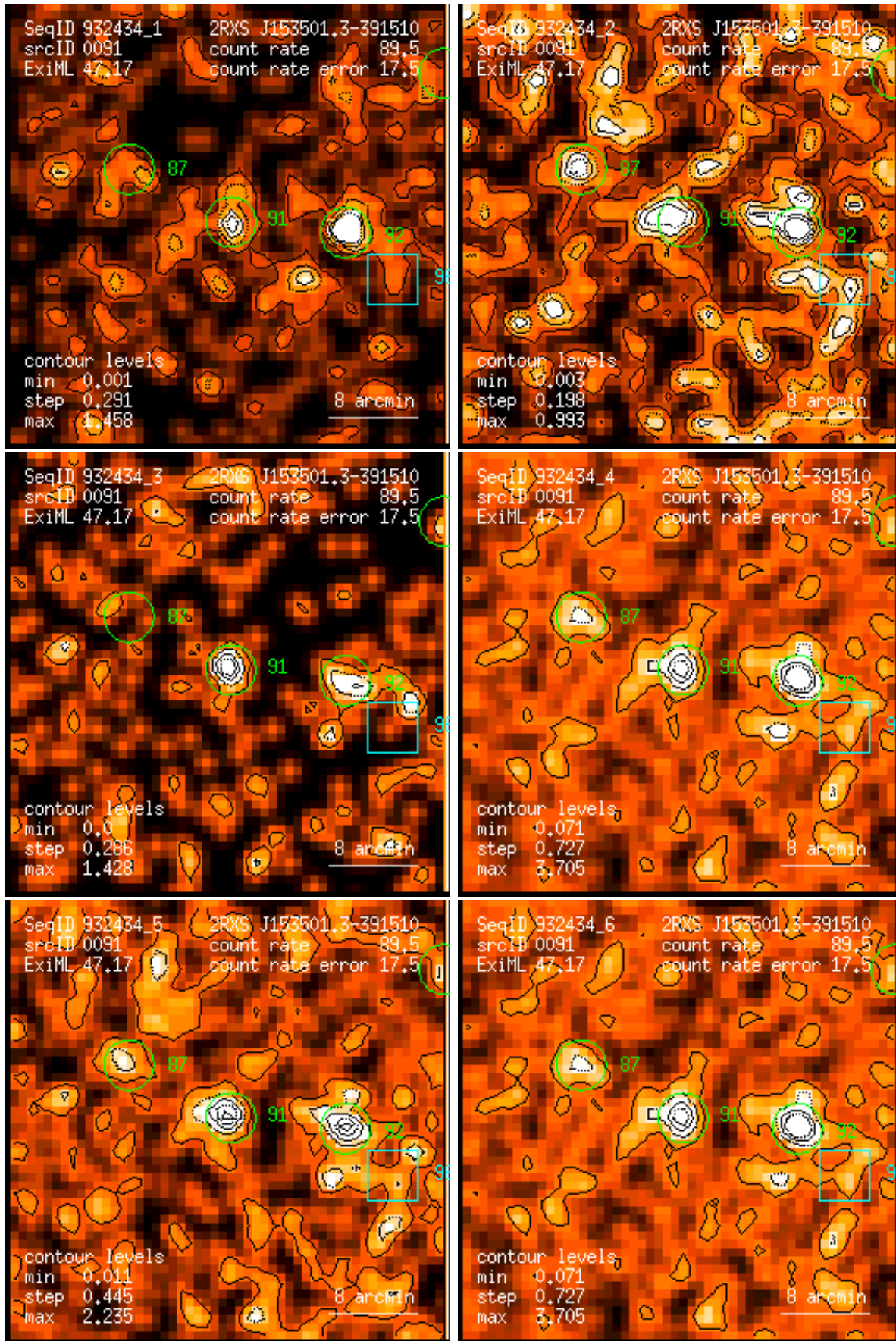
Figure 91: RASS 932434: detection 0091: band rate images, Gaussian filter: (1) PSPC channels 11 – 41, (2) 52 – 90, (3) 91 – 201, (4) 11 – 235, (5) 52 – 201, (6) 11 – 201. Broad band rates in counts/ks. Band rate contour levels in counts/ks/arcmin 2 .
