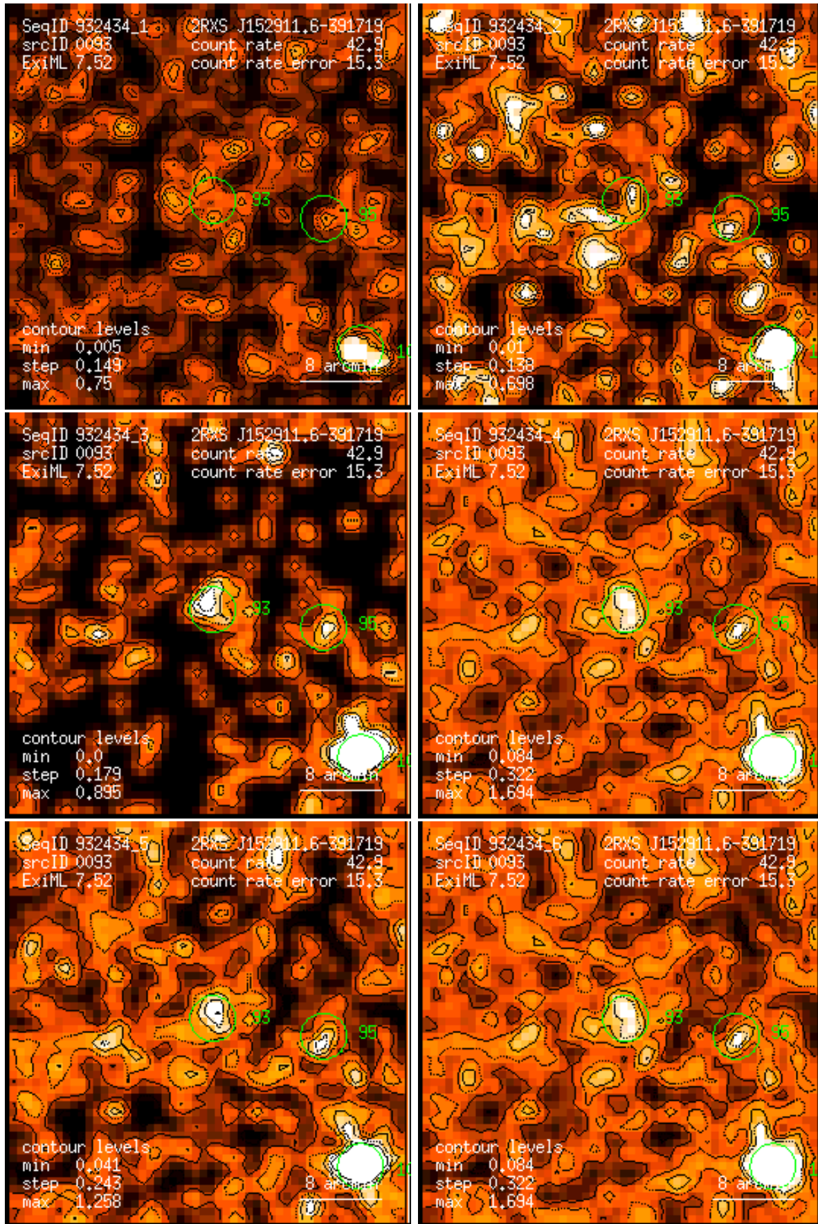
Figure 93: RASS 932434: detection 0093: band rate images, Gaussian filter: (1) PSPC channels 11 – 41, (2) 52 – 90, (3) 91 – 201, (4) 11 – 235, (5) 52 – 201, (6) 11 – 201. Broad band rates in counts/ks. Band rate contour levels in counts/ks/arcmin 2 .
