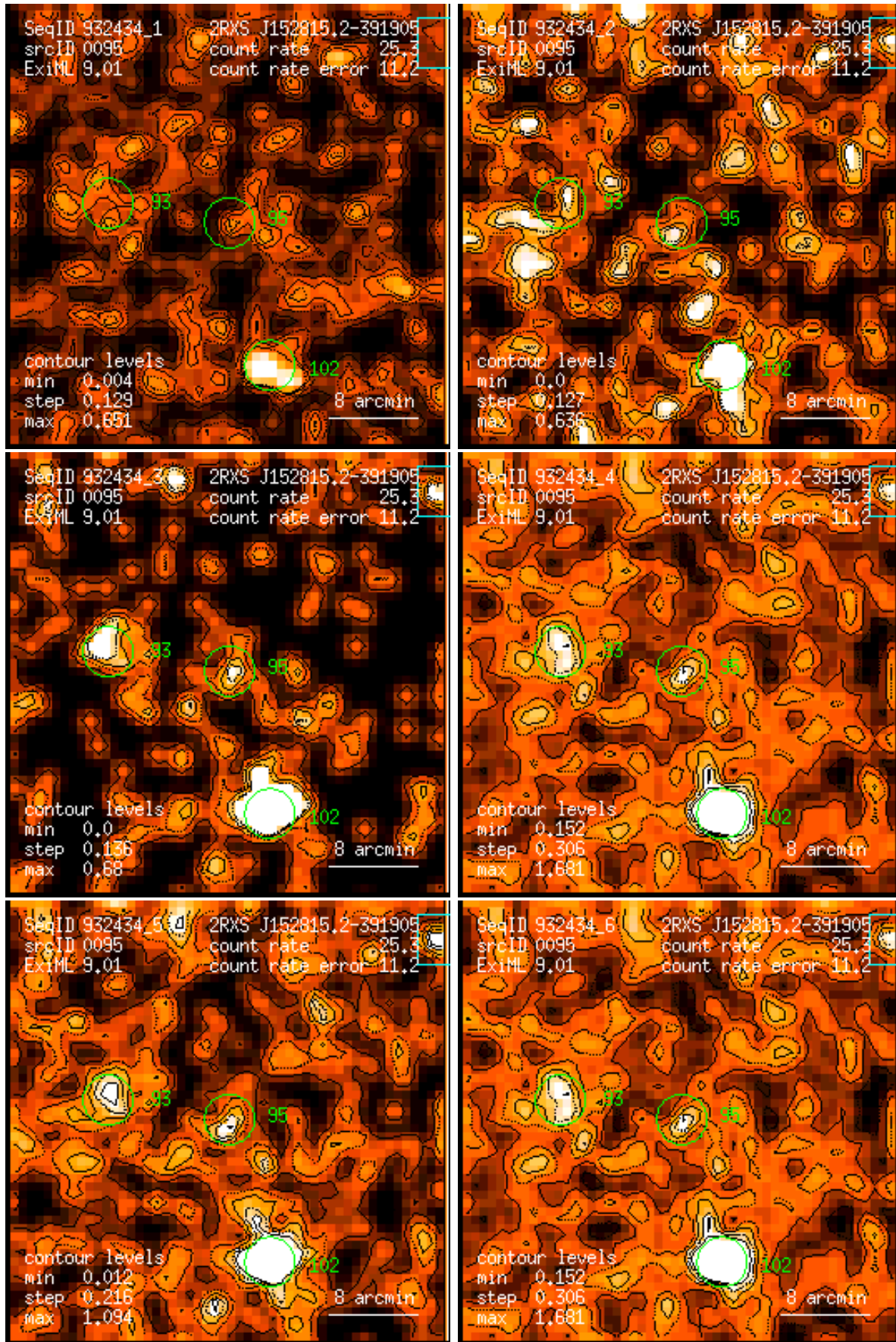
Figure 95: RASS 932434: detection 0095: band rate images, Gaussian filter: (1) PSPC channels 11 – 41, (2) 52 – 90, (3) 91 – 201, (4) 11 – 235, (5) 52 – 201, (6) 11 – 201. Broad band rates in counts/ks. Band rate contour levels in counts/ks/arcmin 2 .
